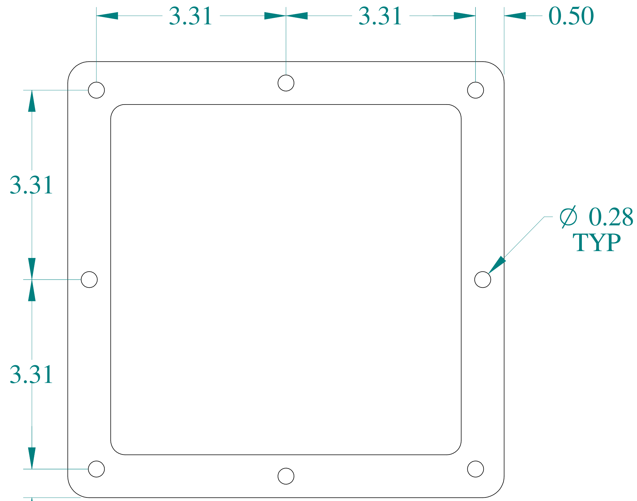
FRONT VIEW
