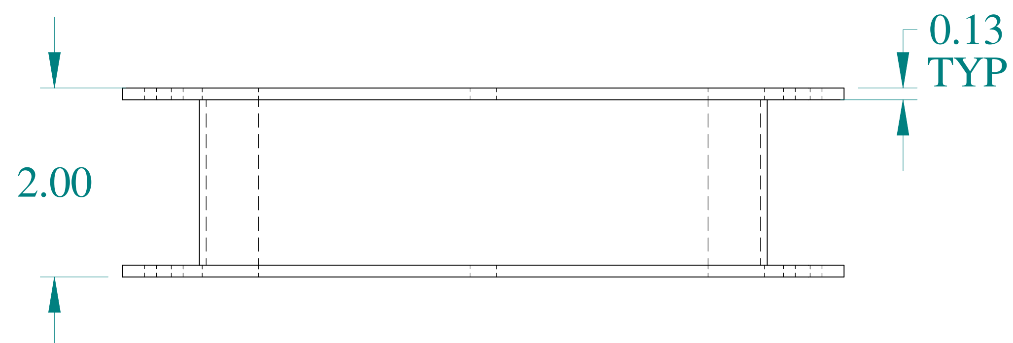
BOTTOM VIEW
