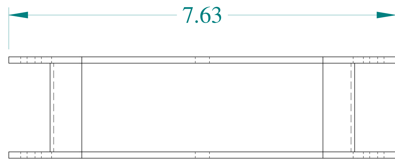
TOP VIEW
