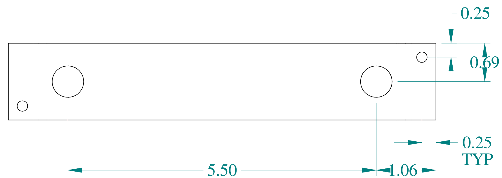
BOTTOM VIEW
