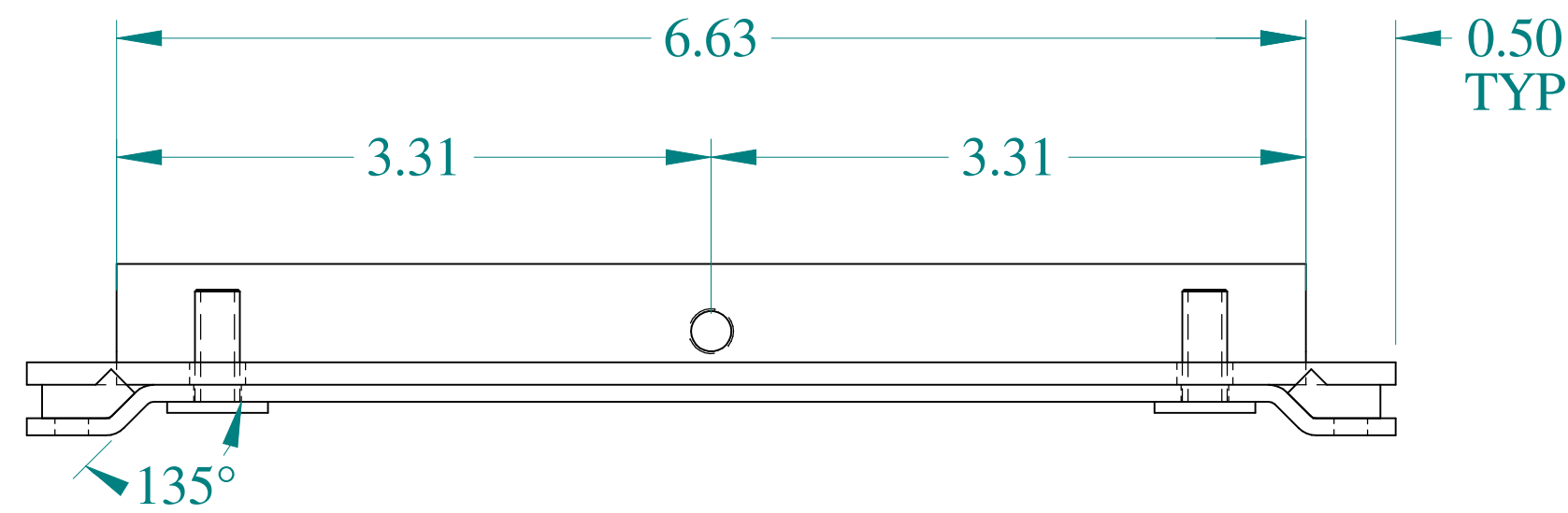
FRONT VIEW
