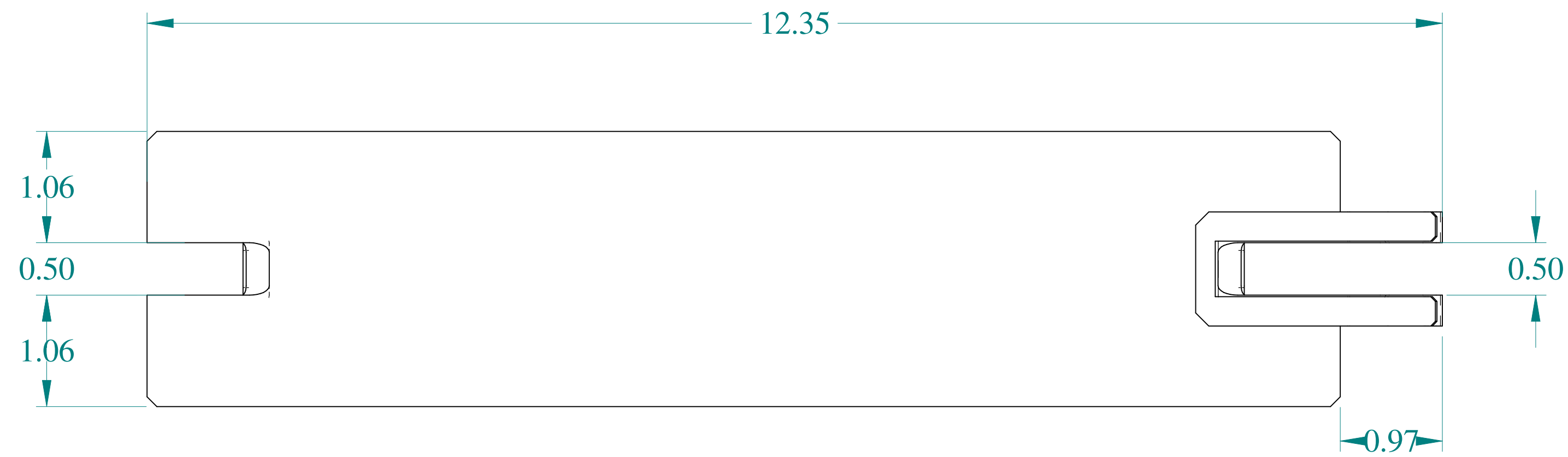
TOP VIEW
