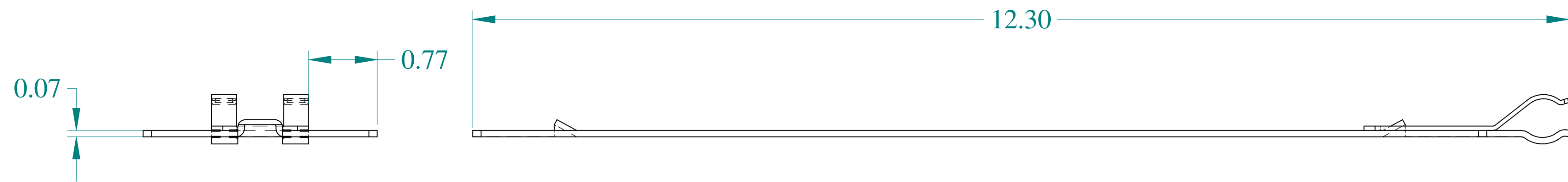
FRONT VIEW
