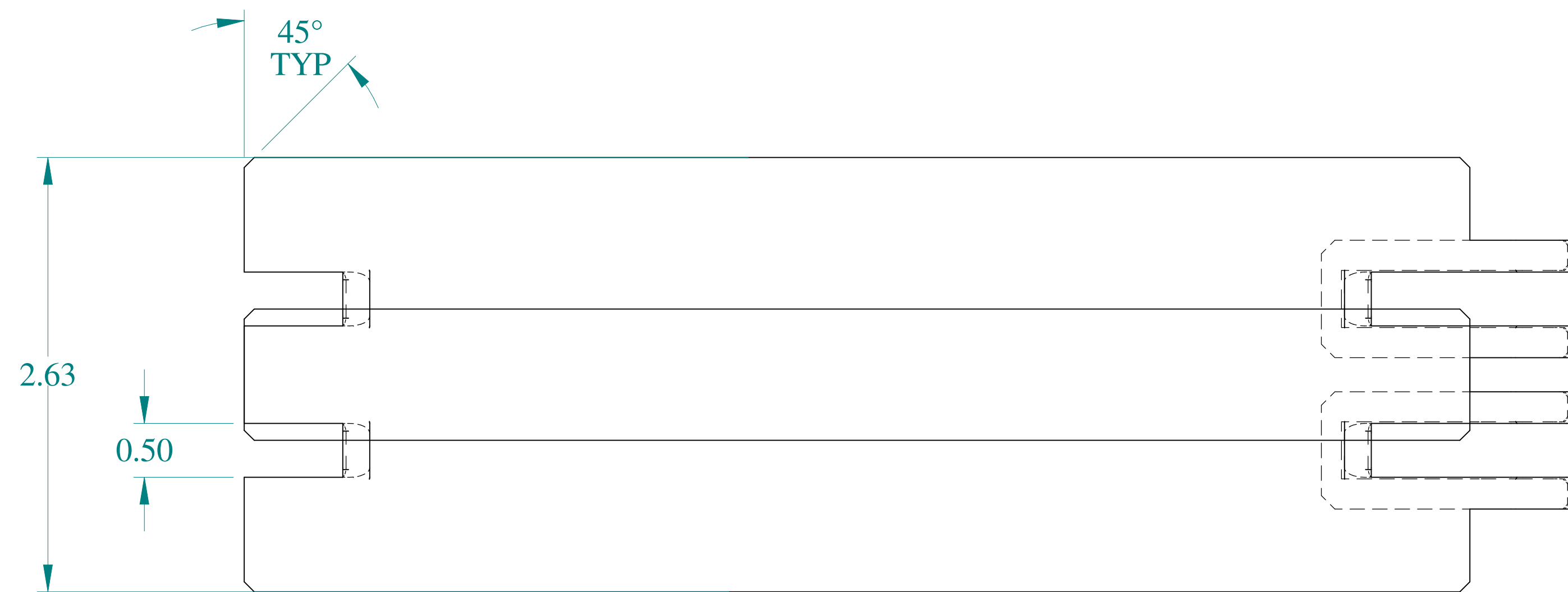
BOTTOM VIEW
