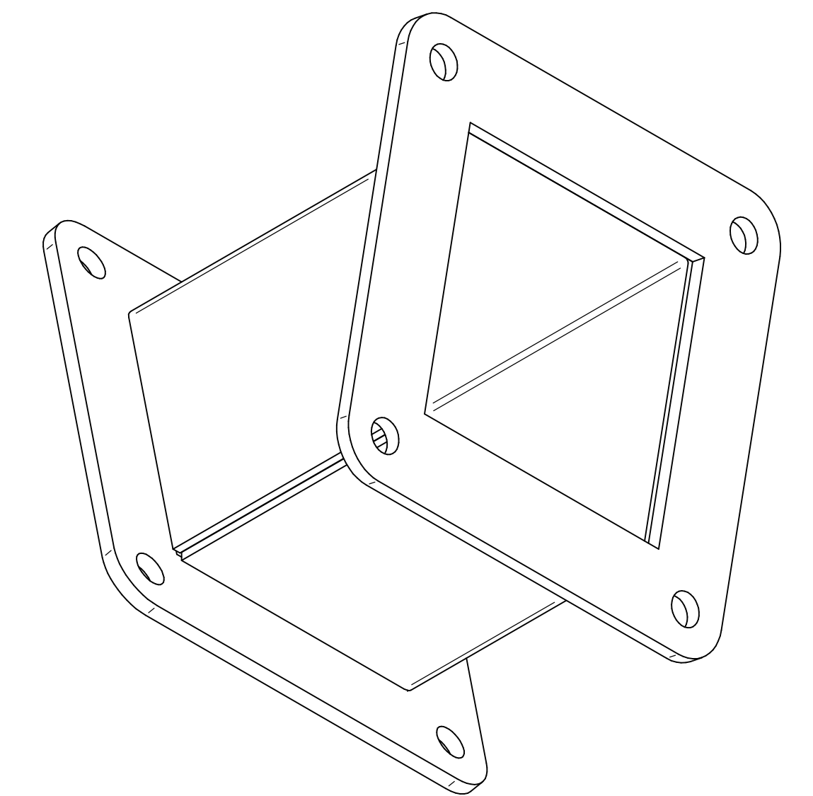
ISOMETRIC VIEWS
