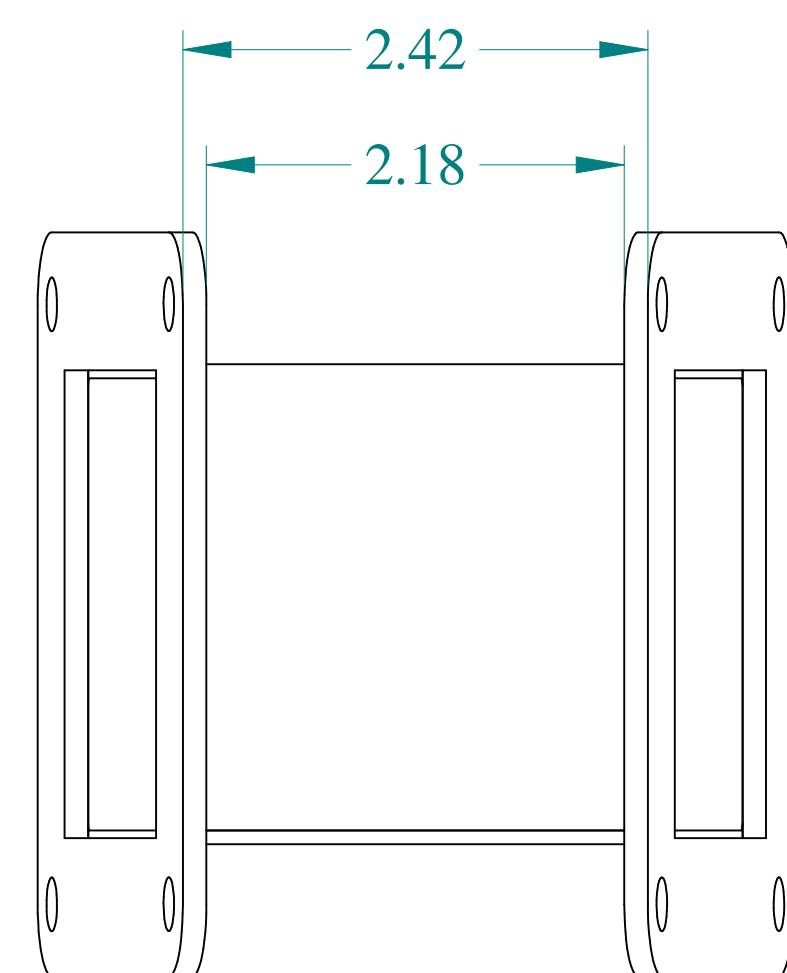
BOTTOM VIEW
