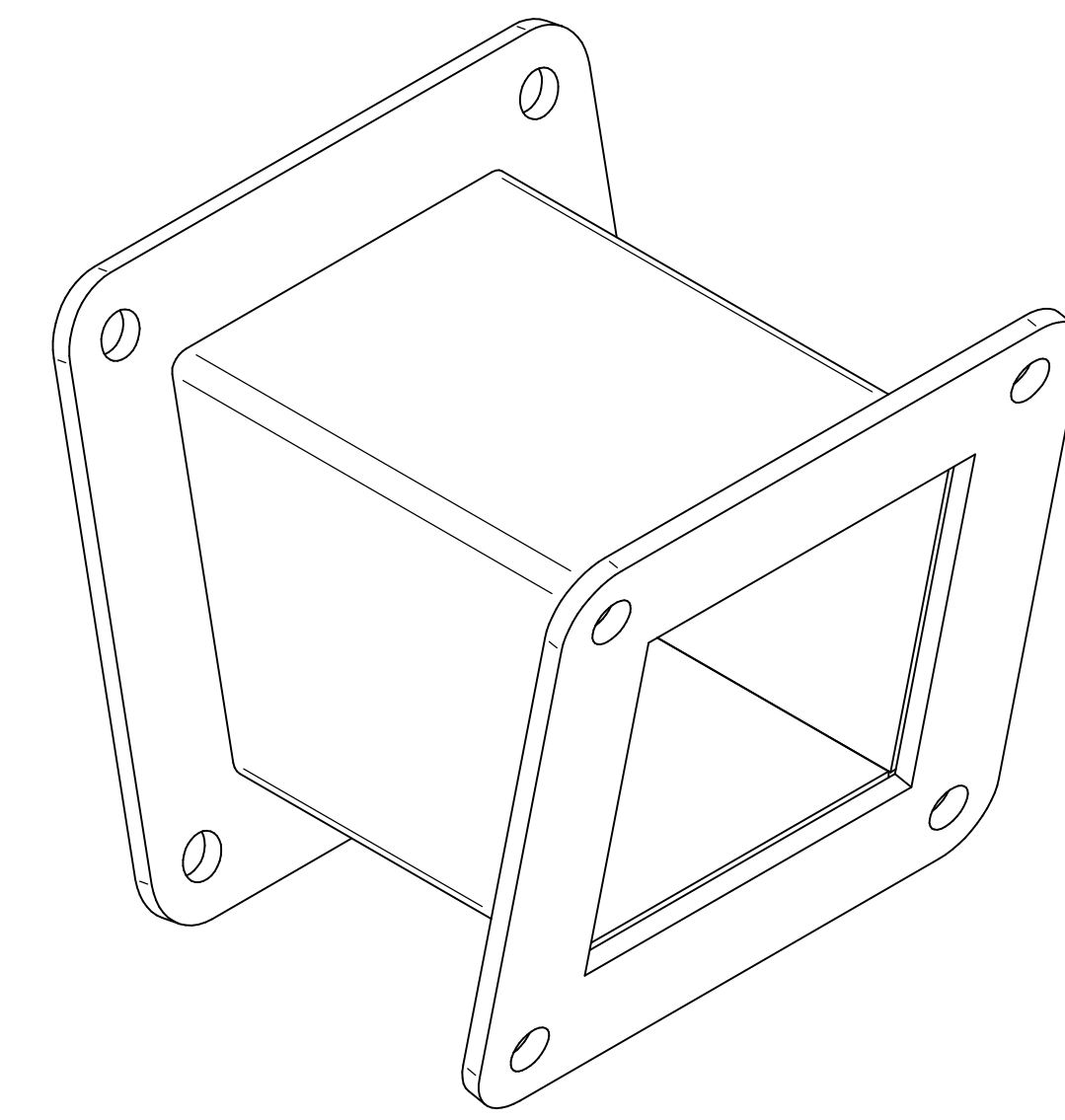
ISOMETRIC VIEWS
