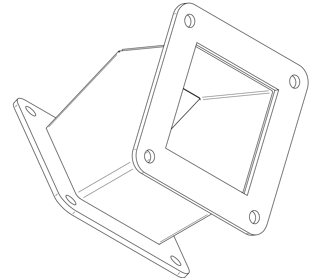
ISOMETRIC VIEWS
