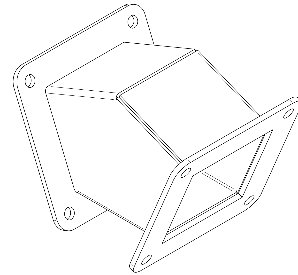
ISOMETRIC VIEWS
