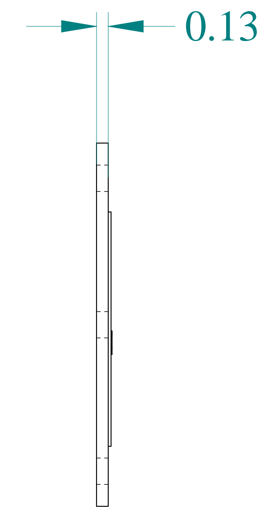
SIDE VIEW
