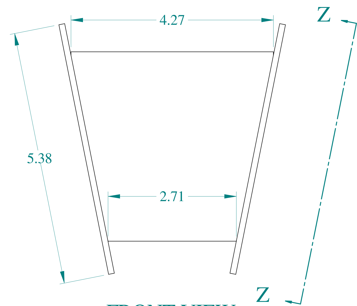
FRONT VIEW
