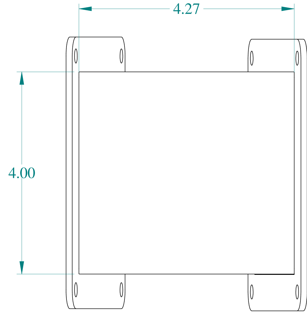
TOP VIEW
