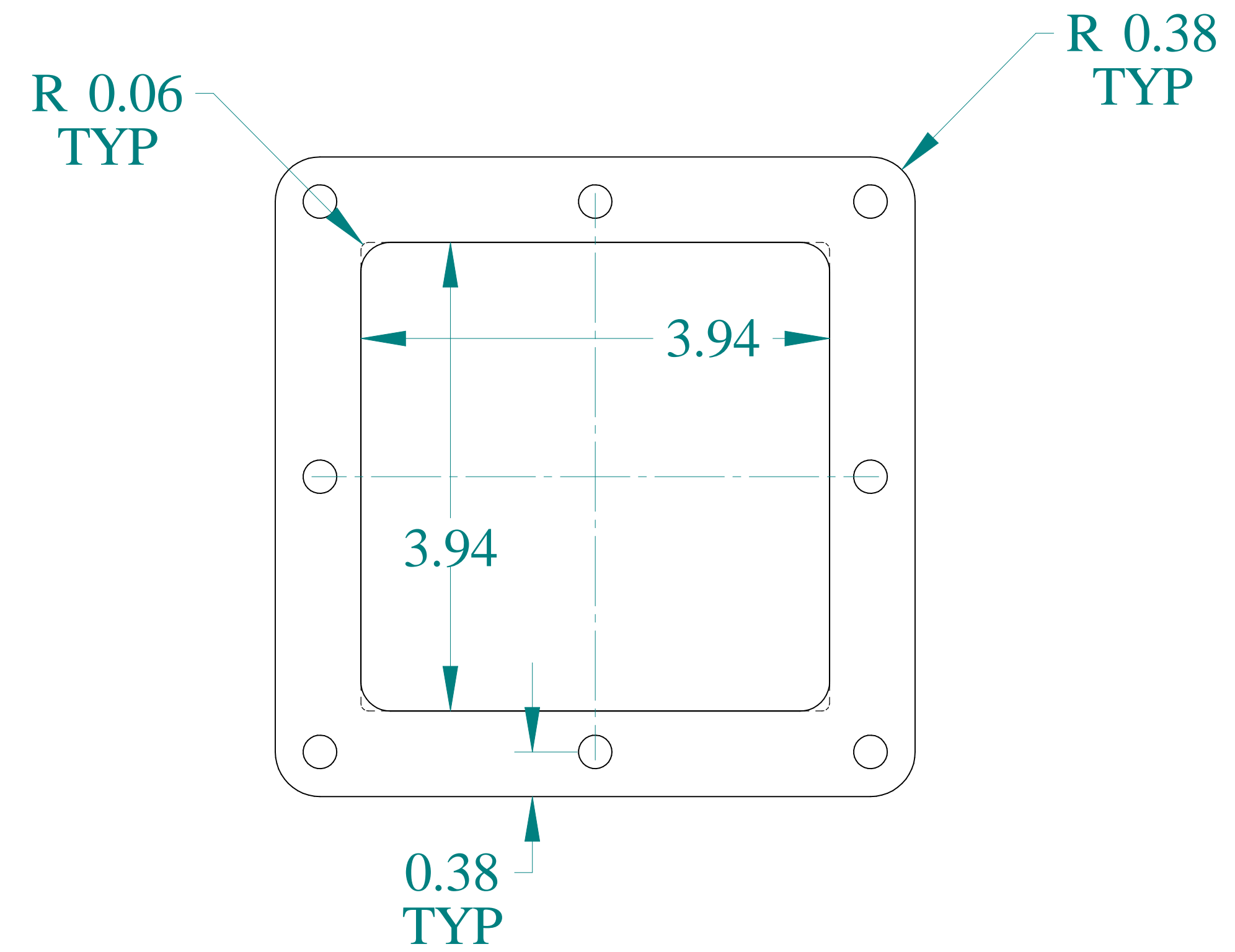
BACK VIEW
