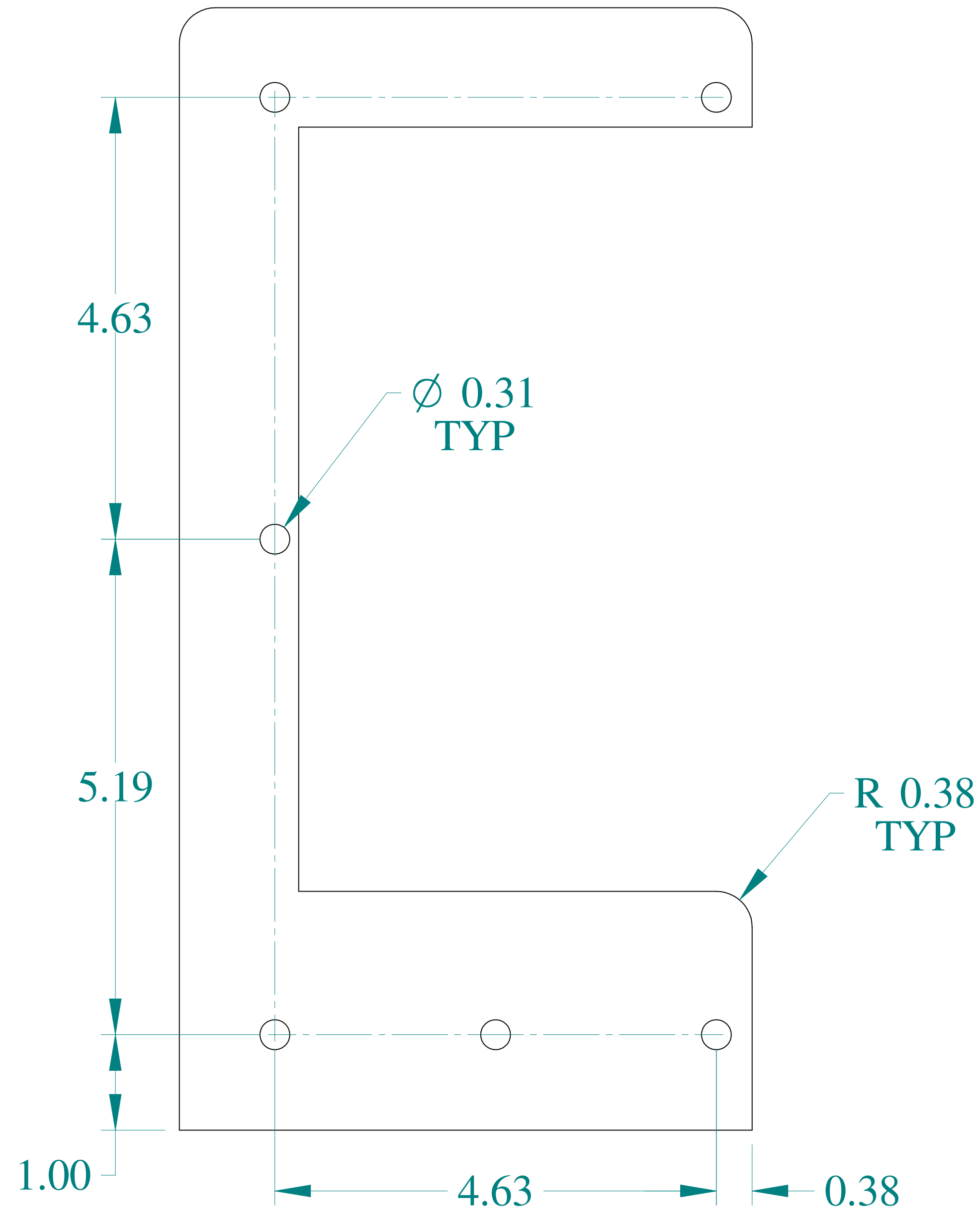
FRONT VIEW
