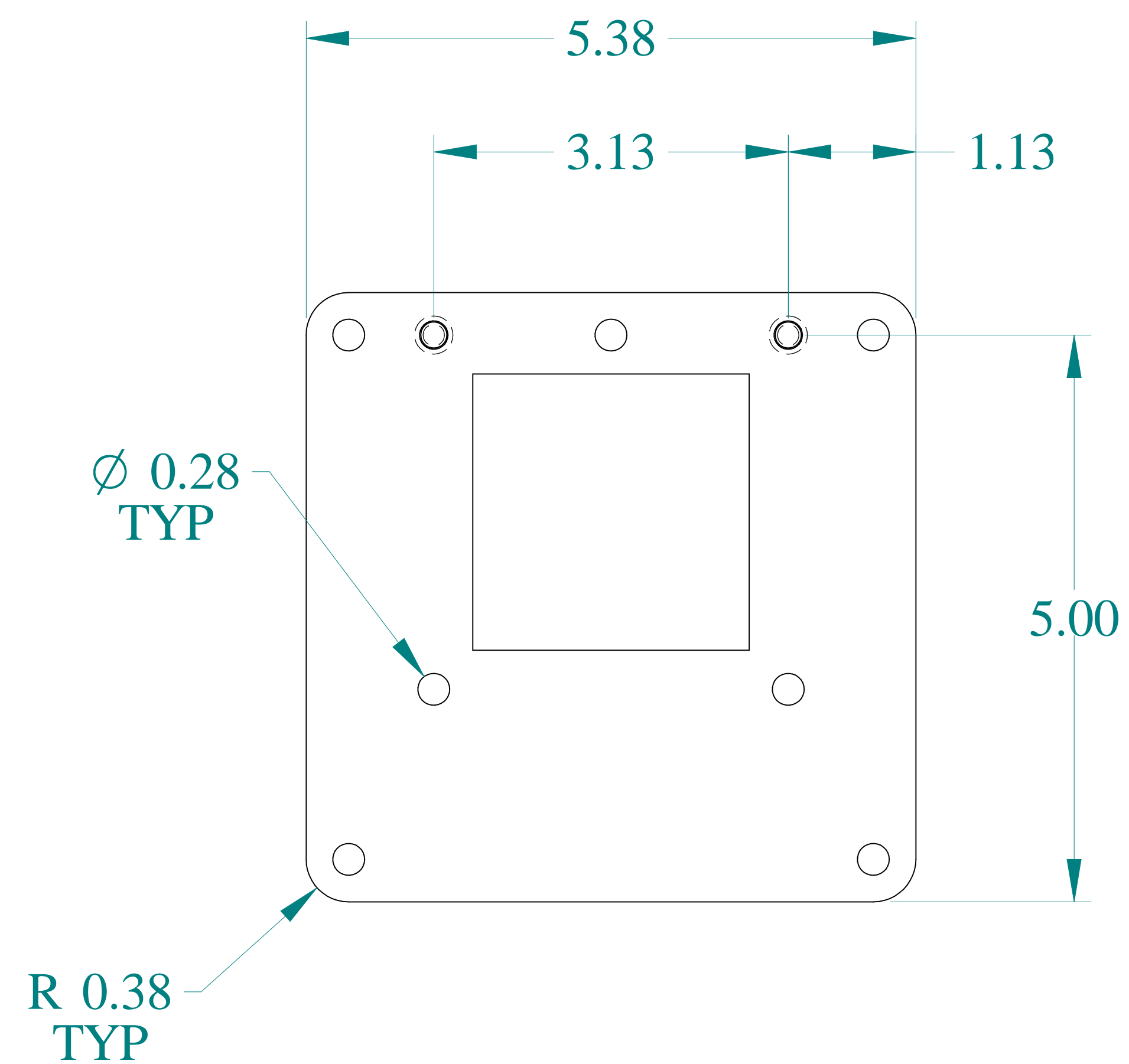
FRONT VIEW
