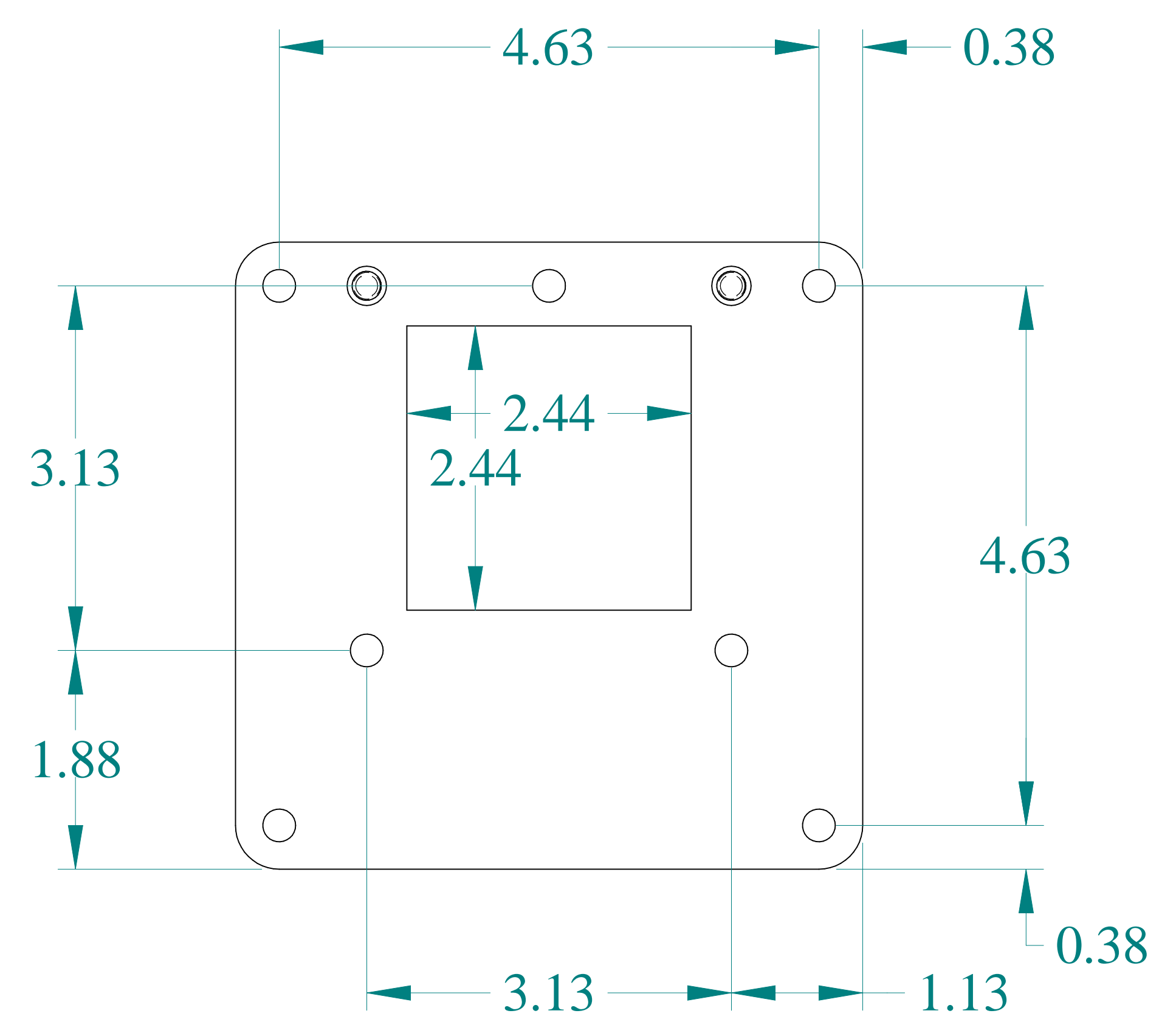
BACK VIEW
