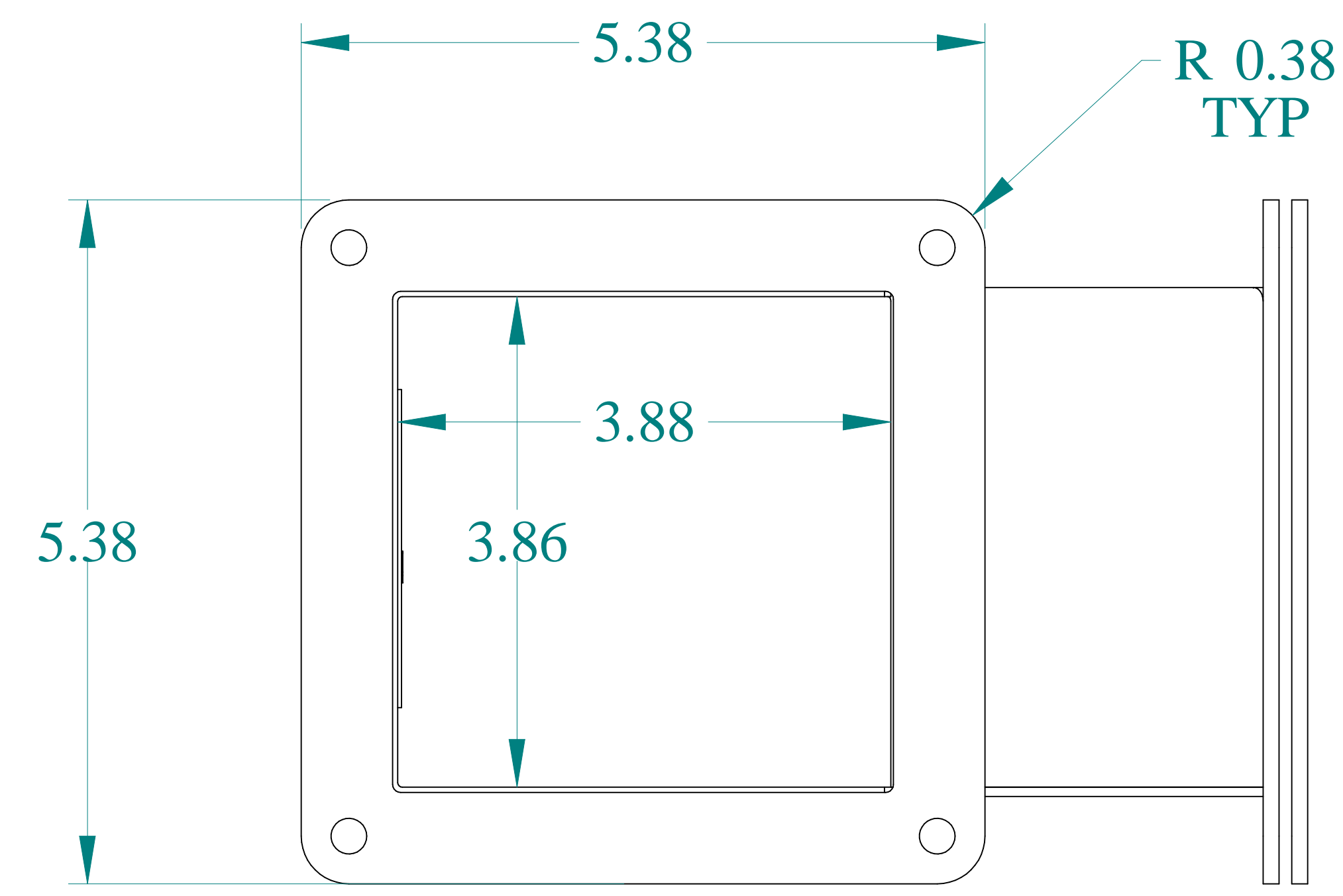
SIDE VIEW
