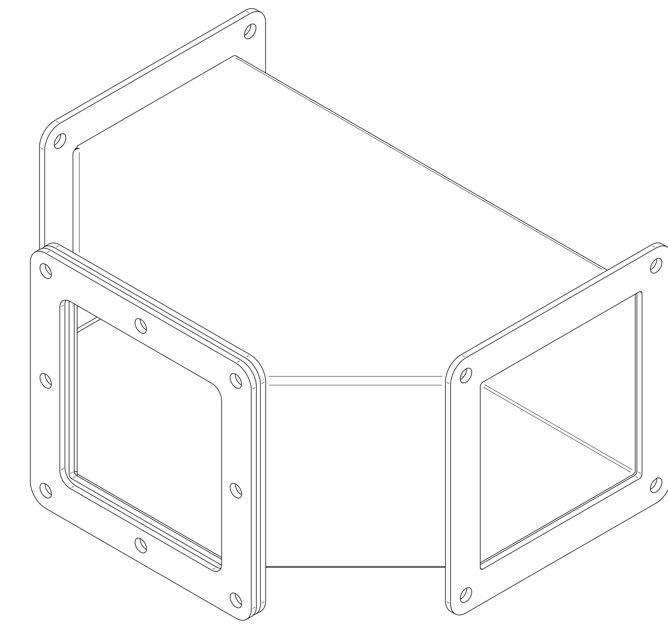
ISOMETRIC VIEWS
