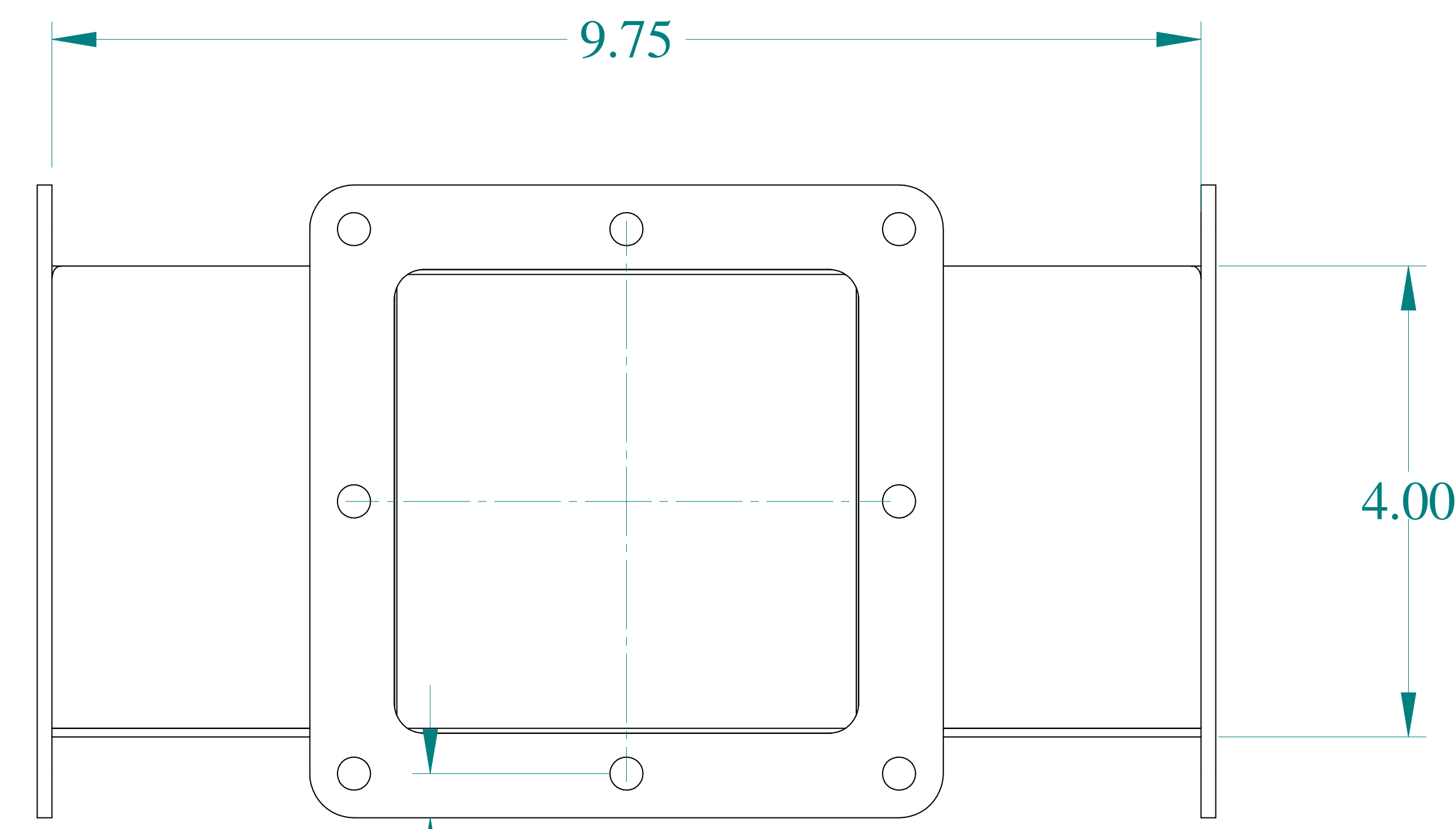
FRONT VIEW
