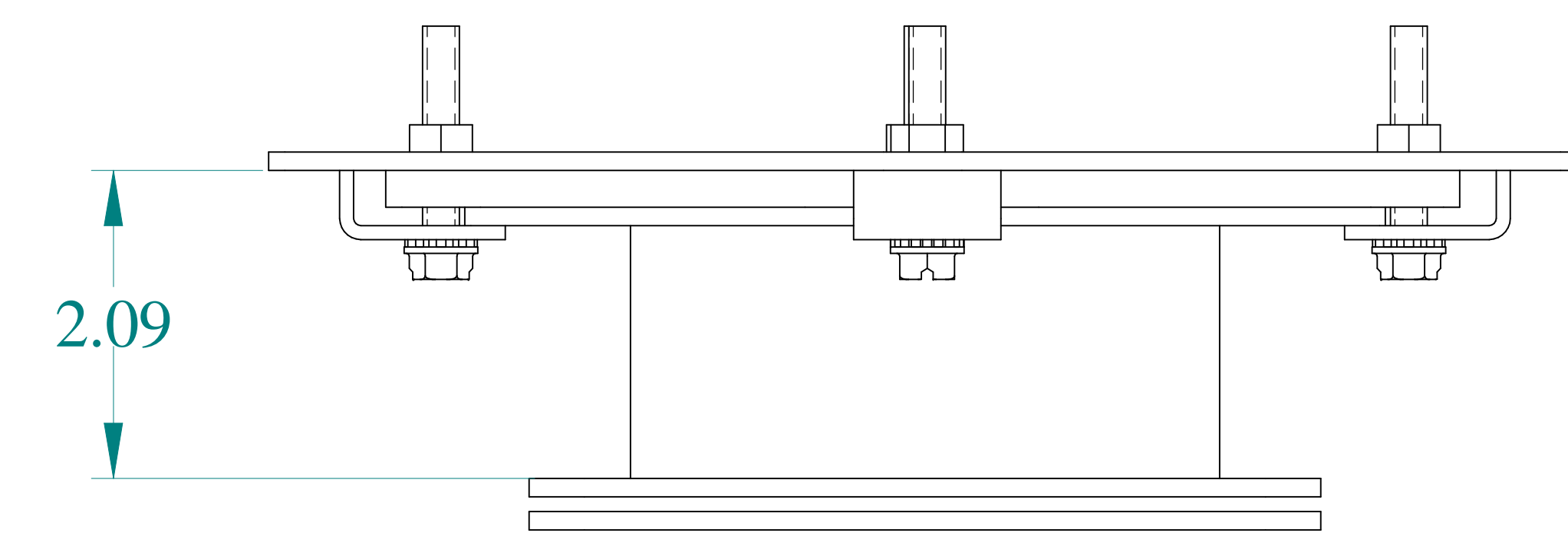
TOP VIEW
