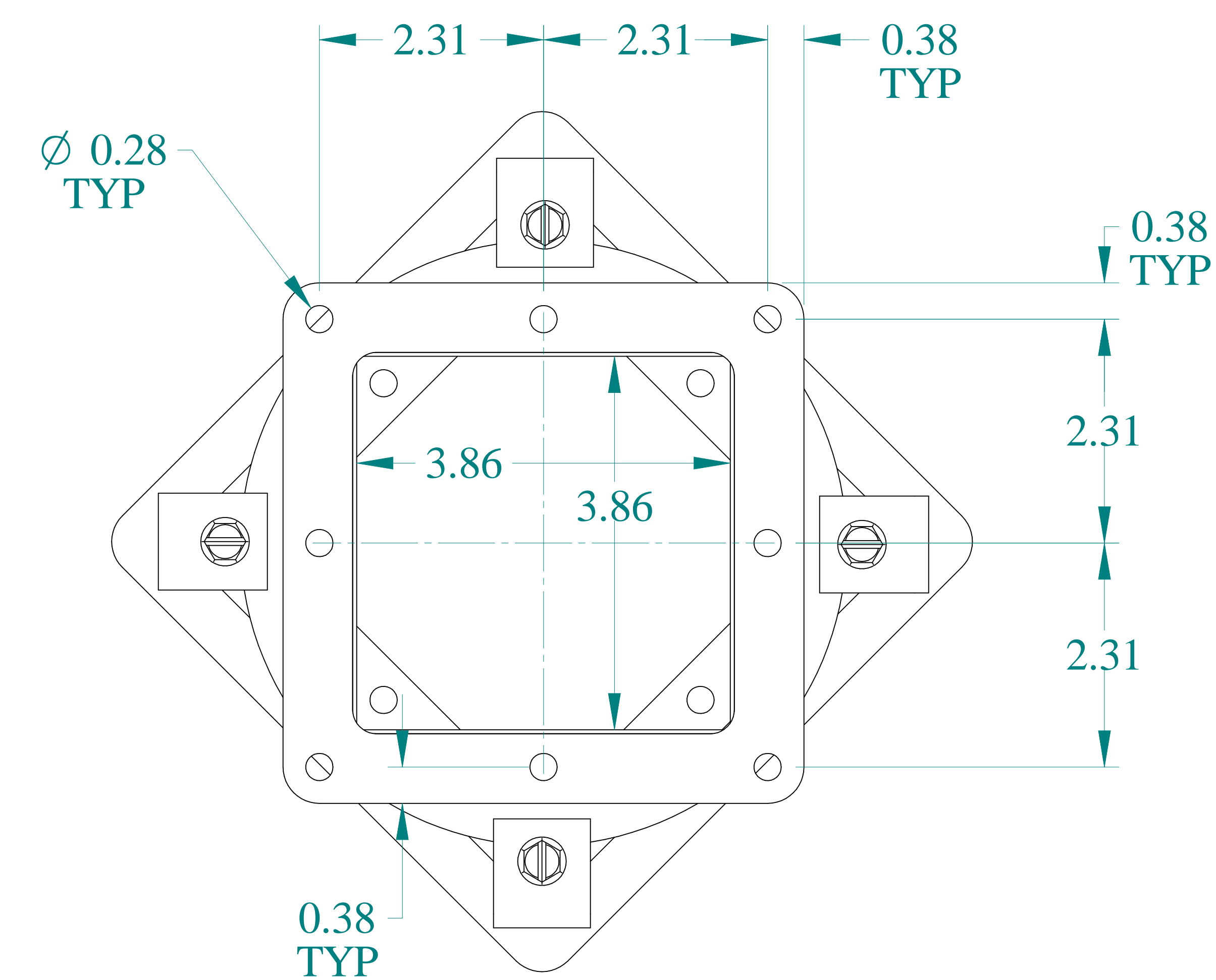
FRONT VIEW
