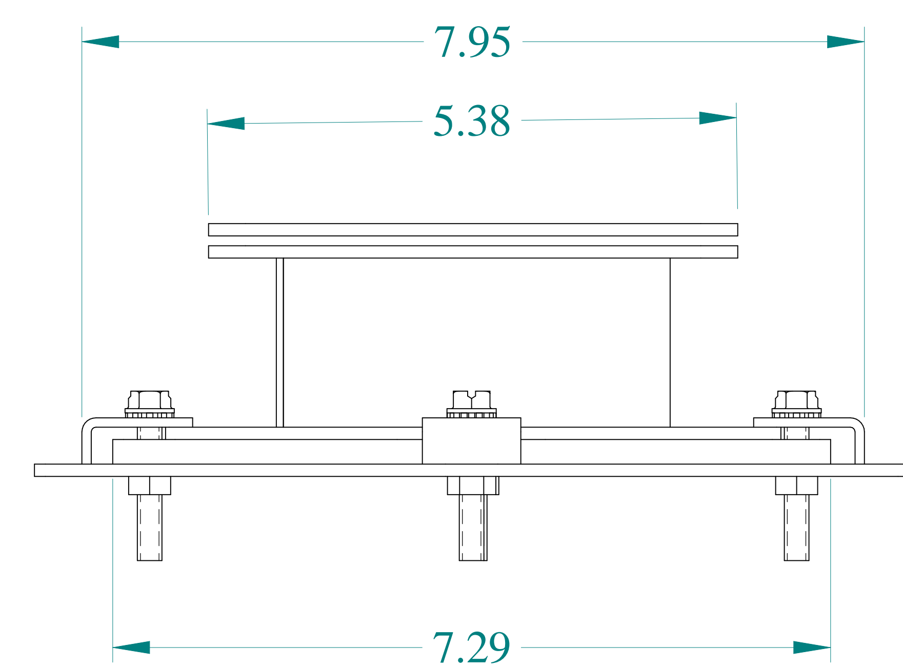
BOTTOM VIEW
