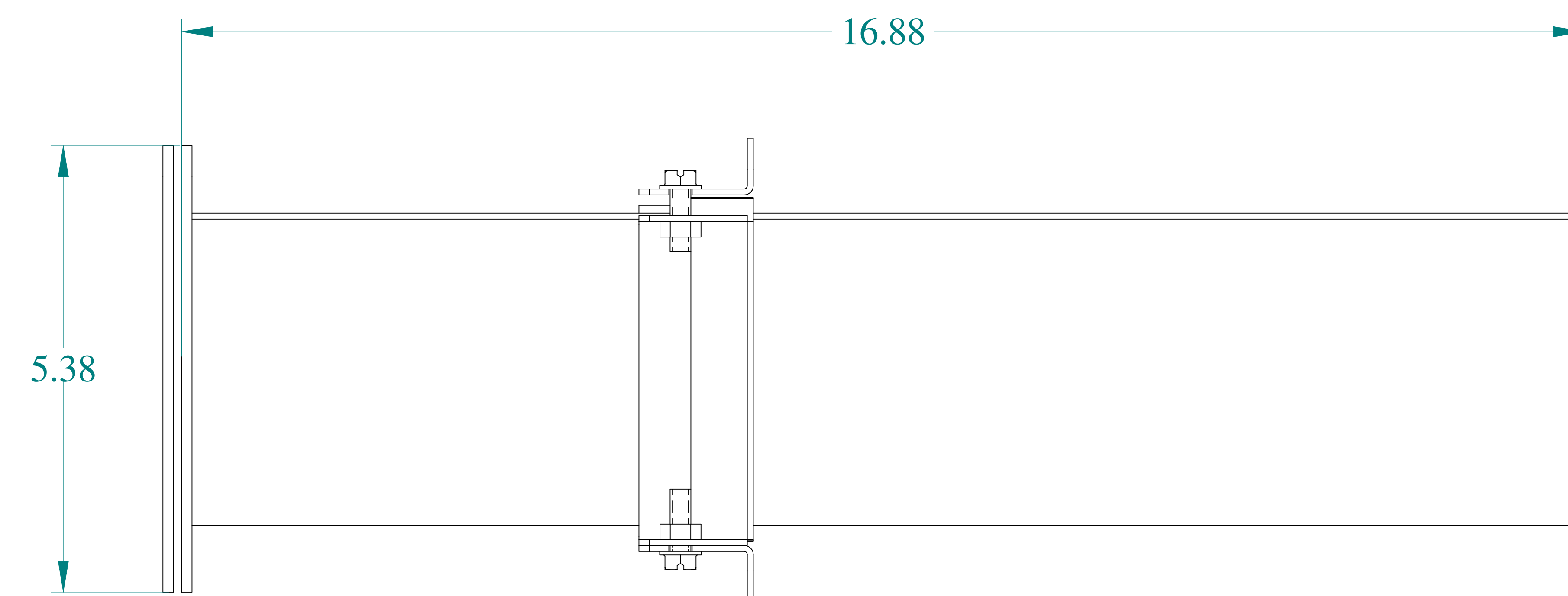
BOTTOM VIEW
