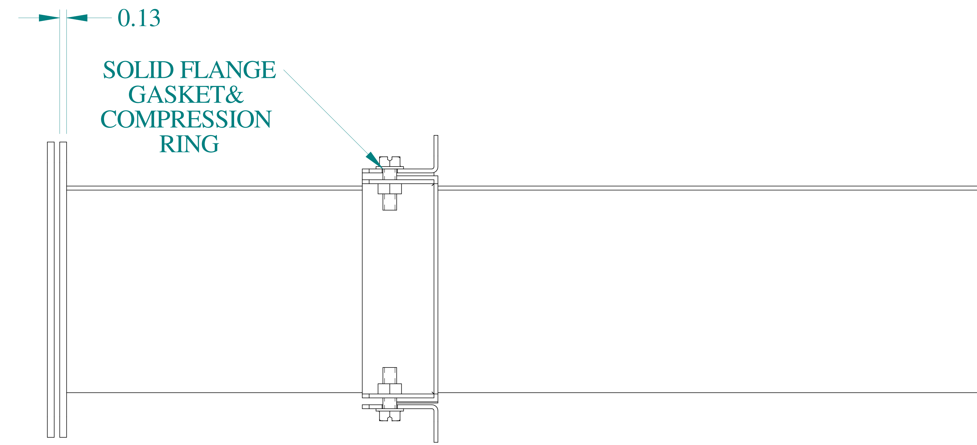
TOP VIEW
