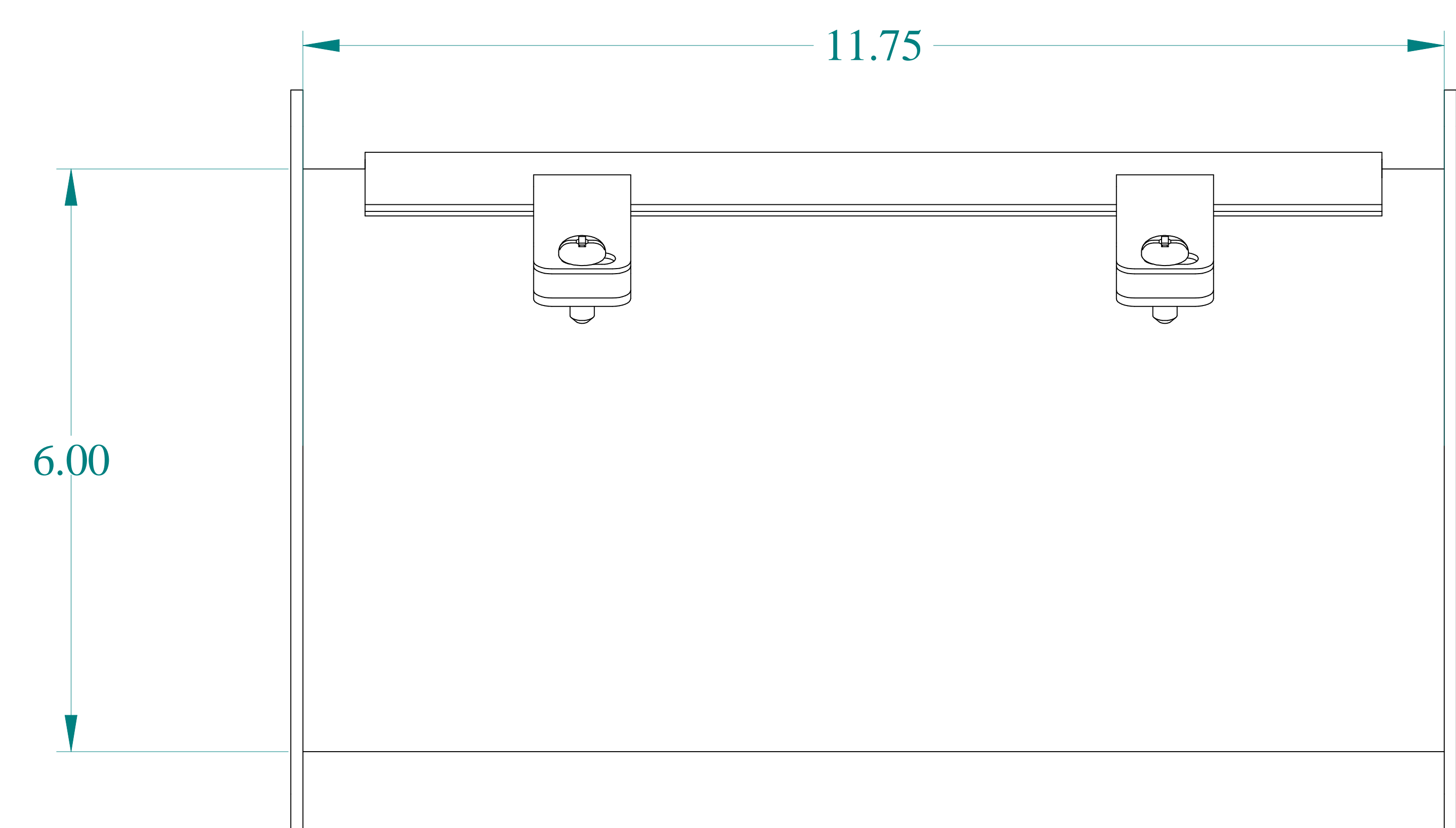
FRONT VIEW
