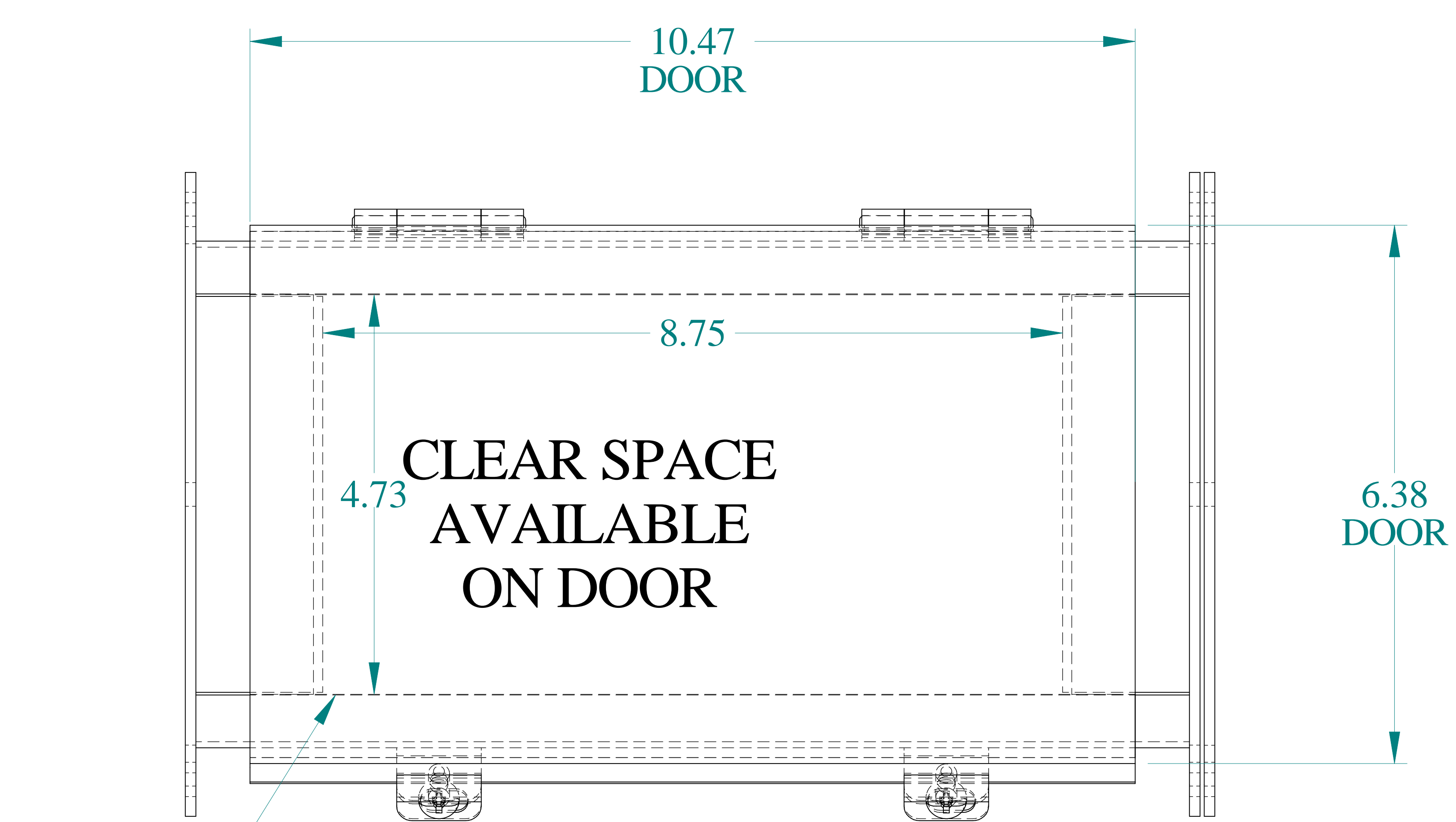
TOP VIEW
