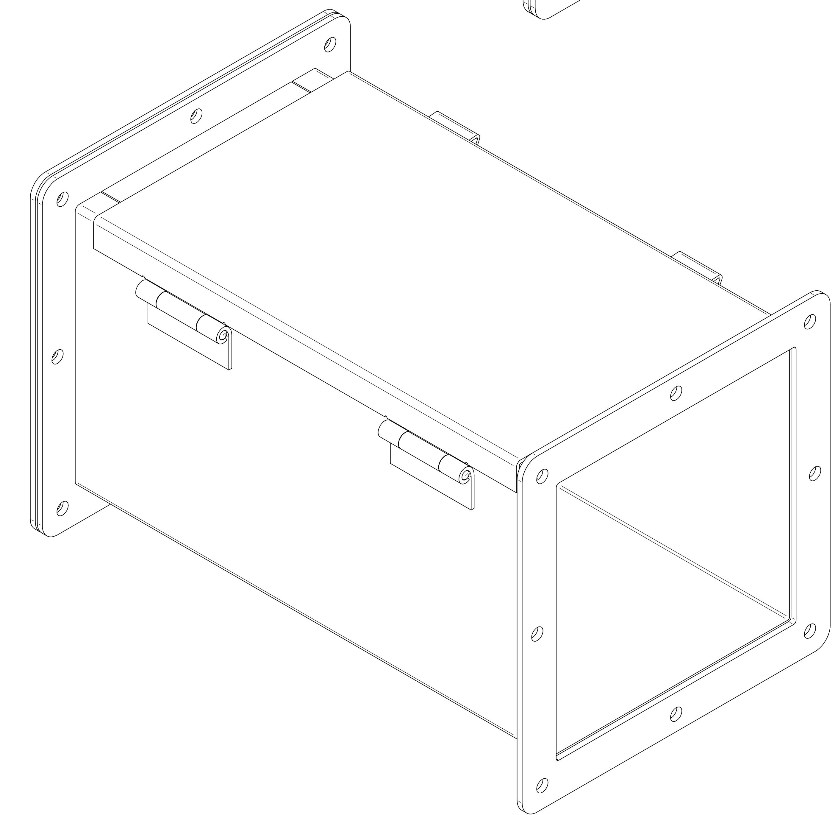
ISOMETRIC VIEWS
