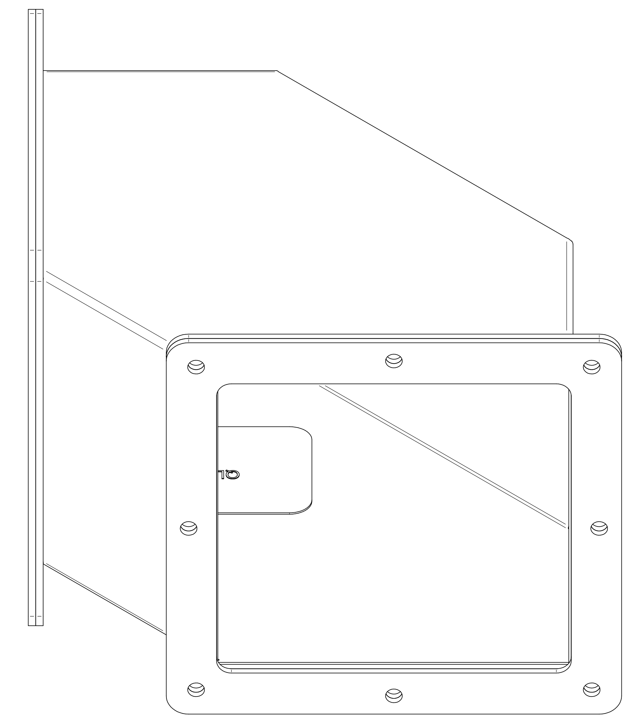
ISOMETRIC VIEWS
