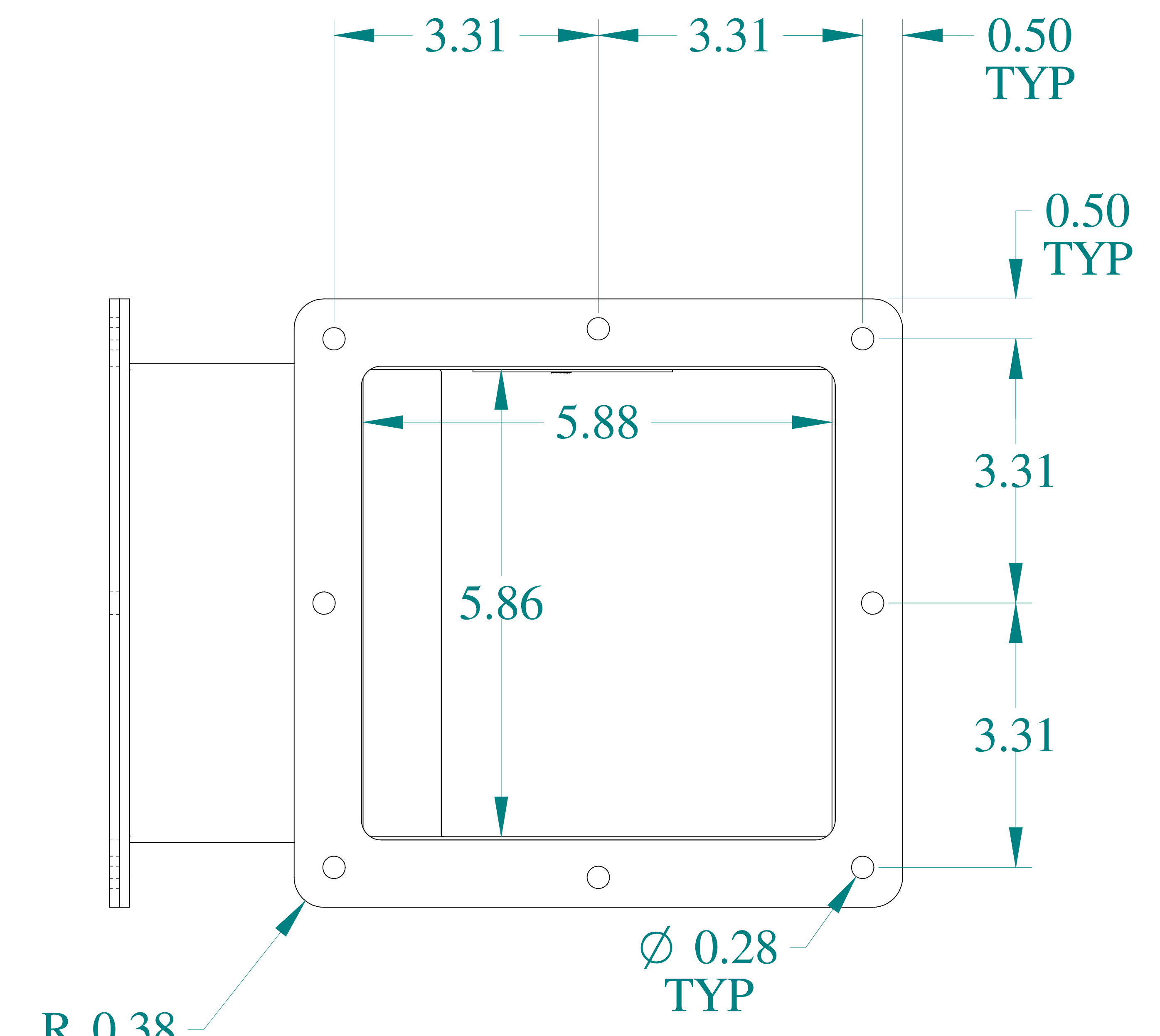
VIEW Z-Z
