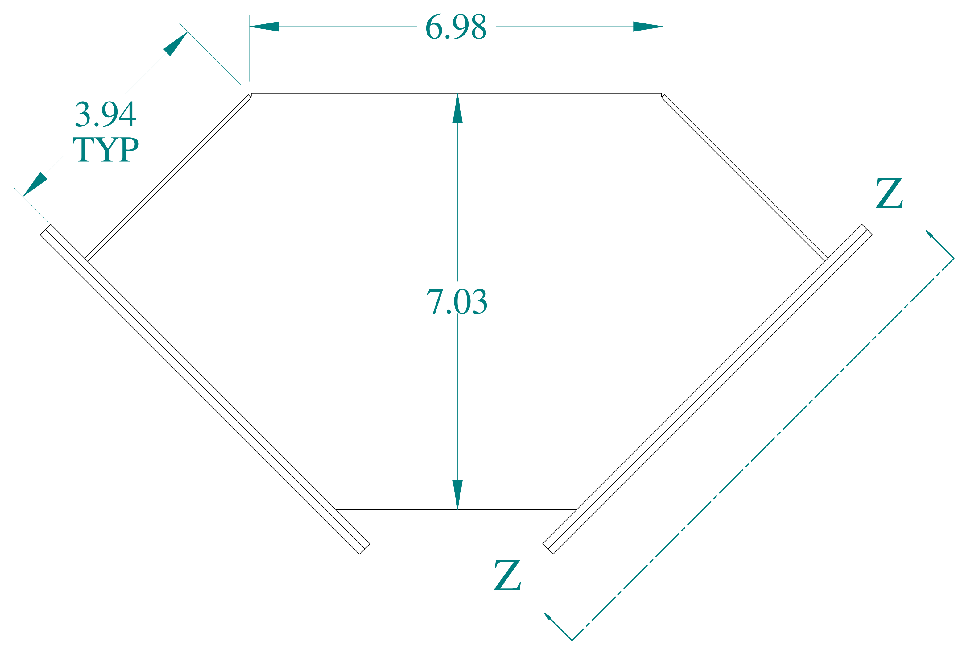
TOP VIEW
