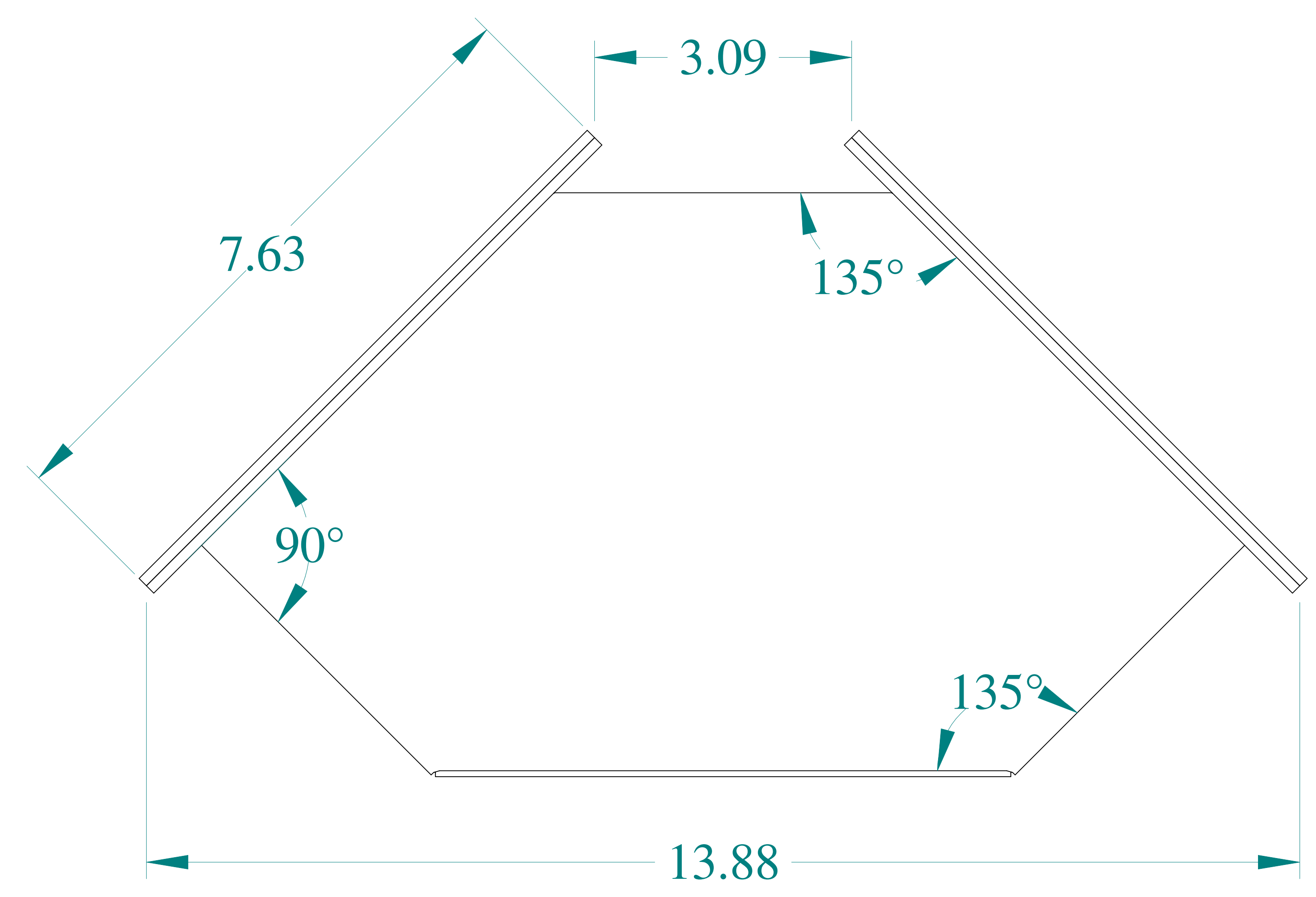
BOTTOM VIEW
