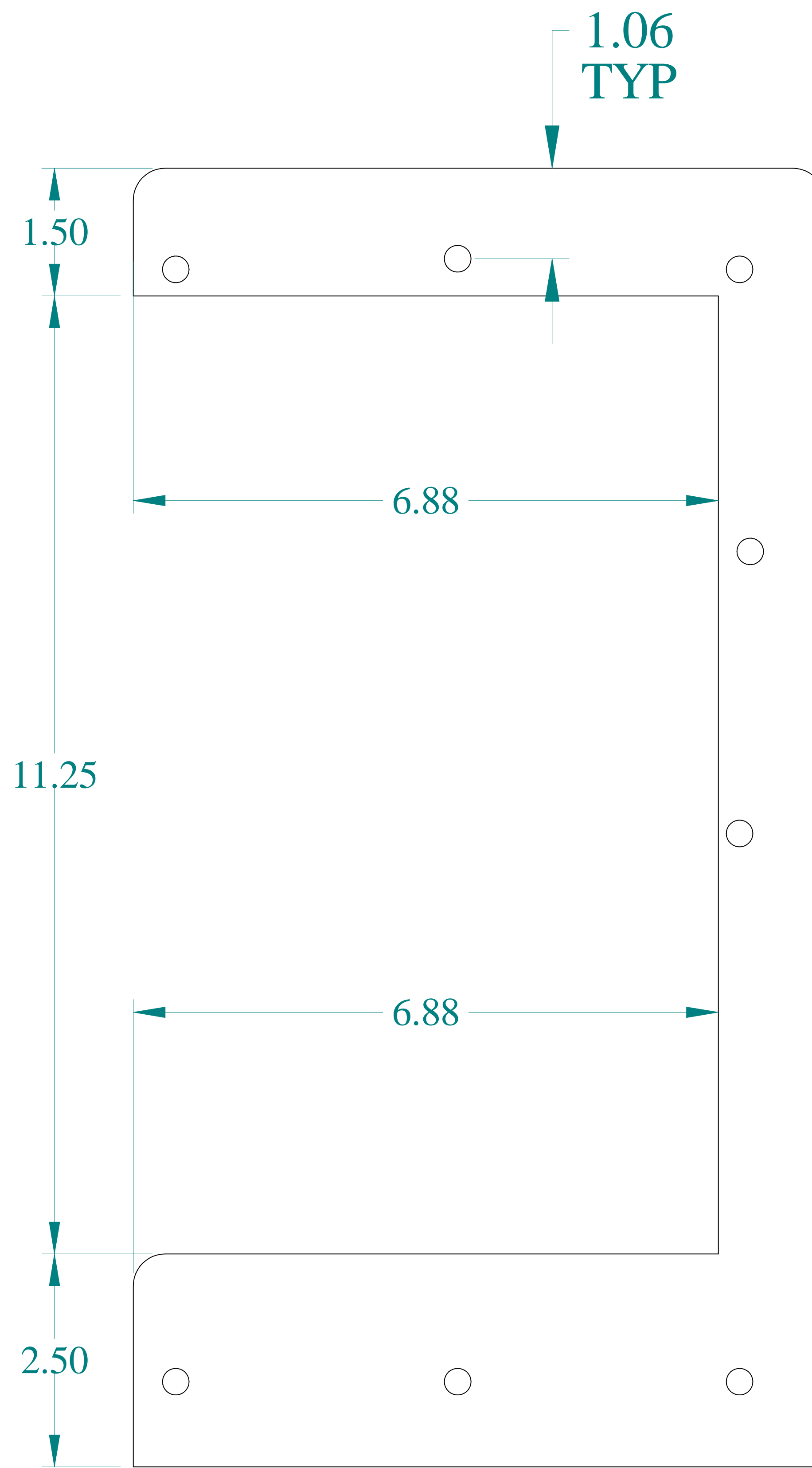
BACK VIEW
