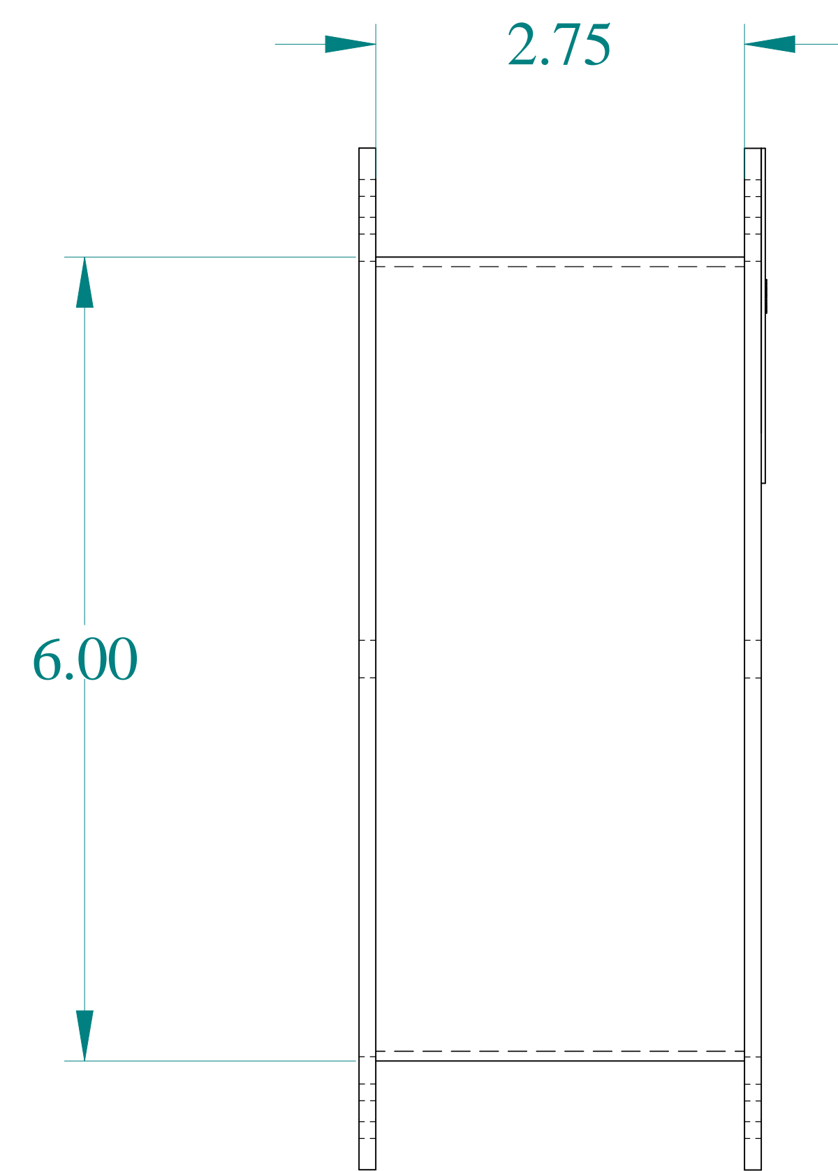
FRONT VIEW
