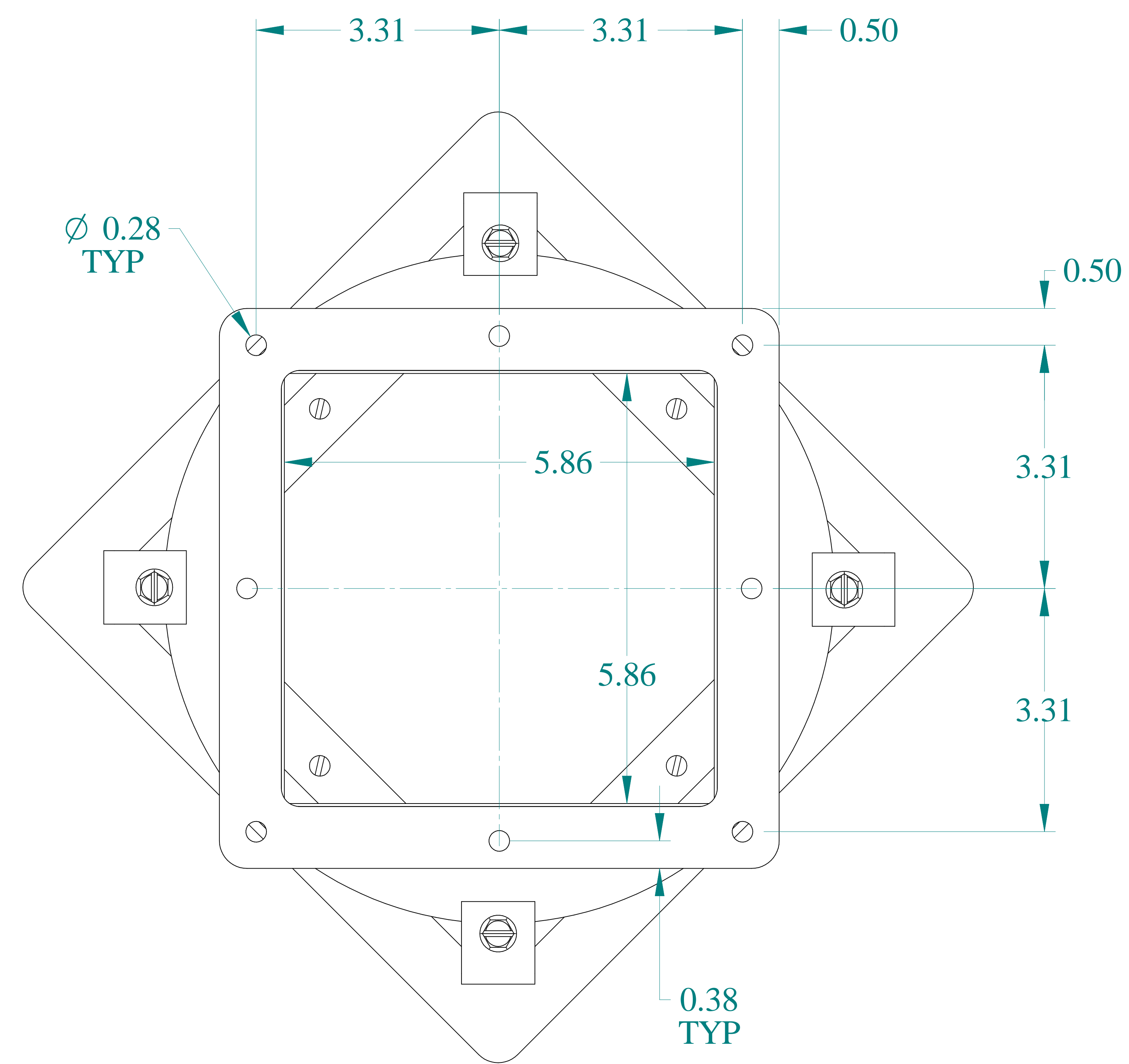
FRONT VIEW
