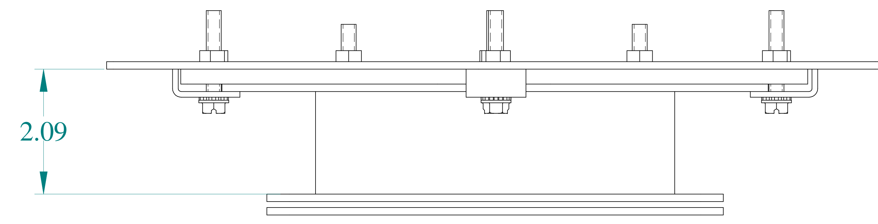
TOP VIEW
