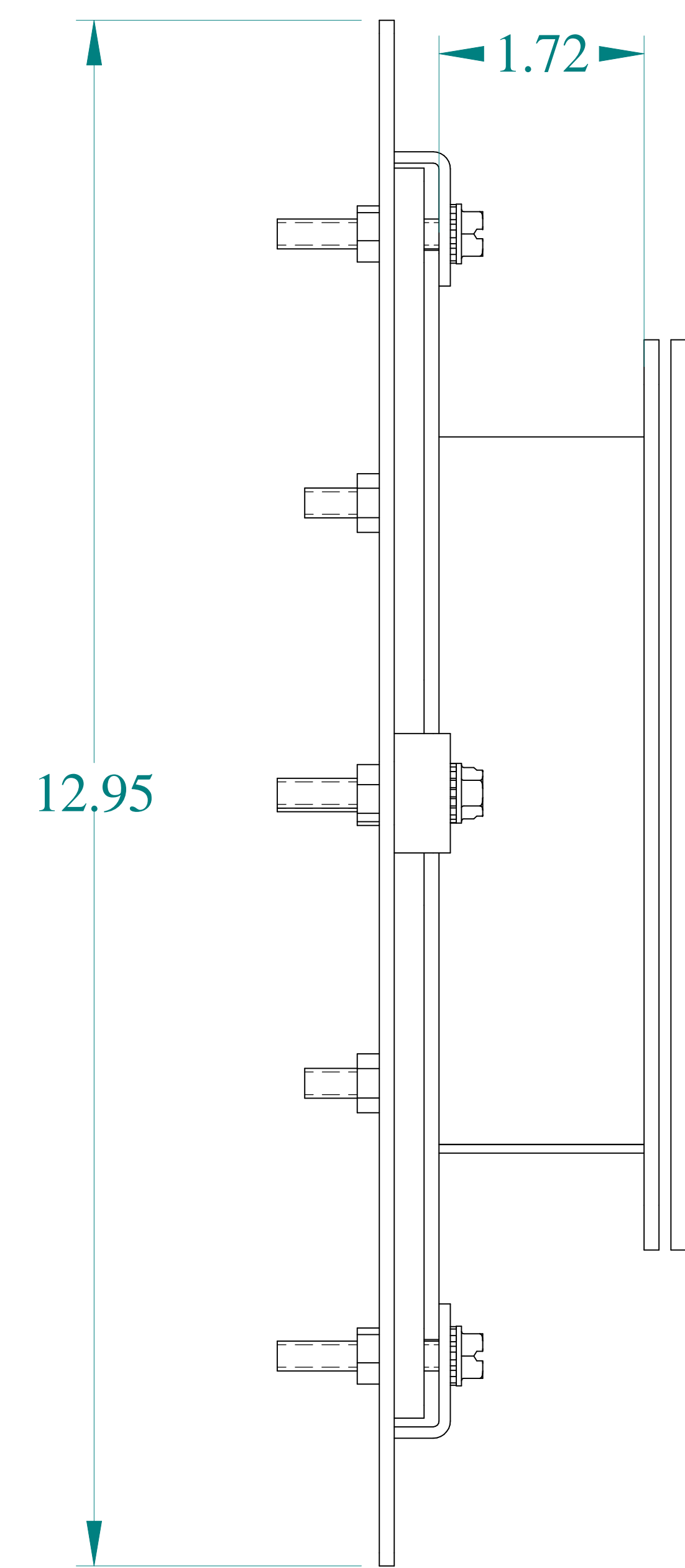
SIDE VIEW
