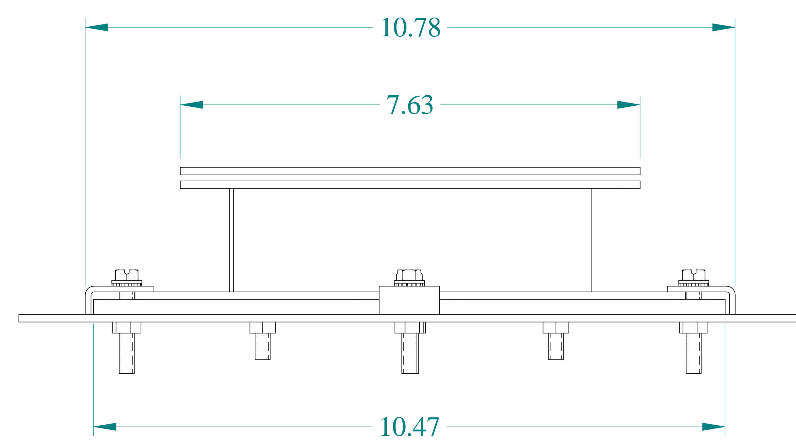
BOTTOM VIEW
