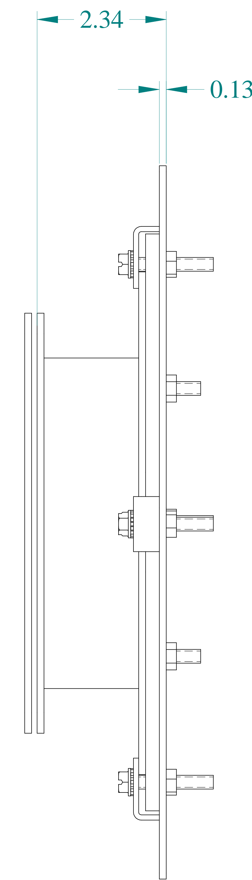
SIDE VIEW
