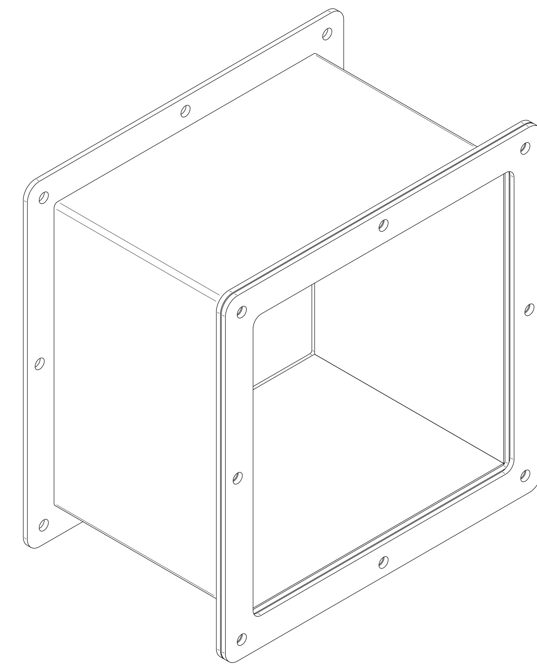
ISOMETRIC VIEWS
