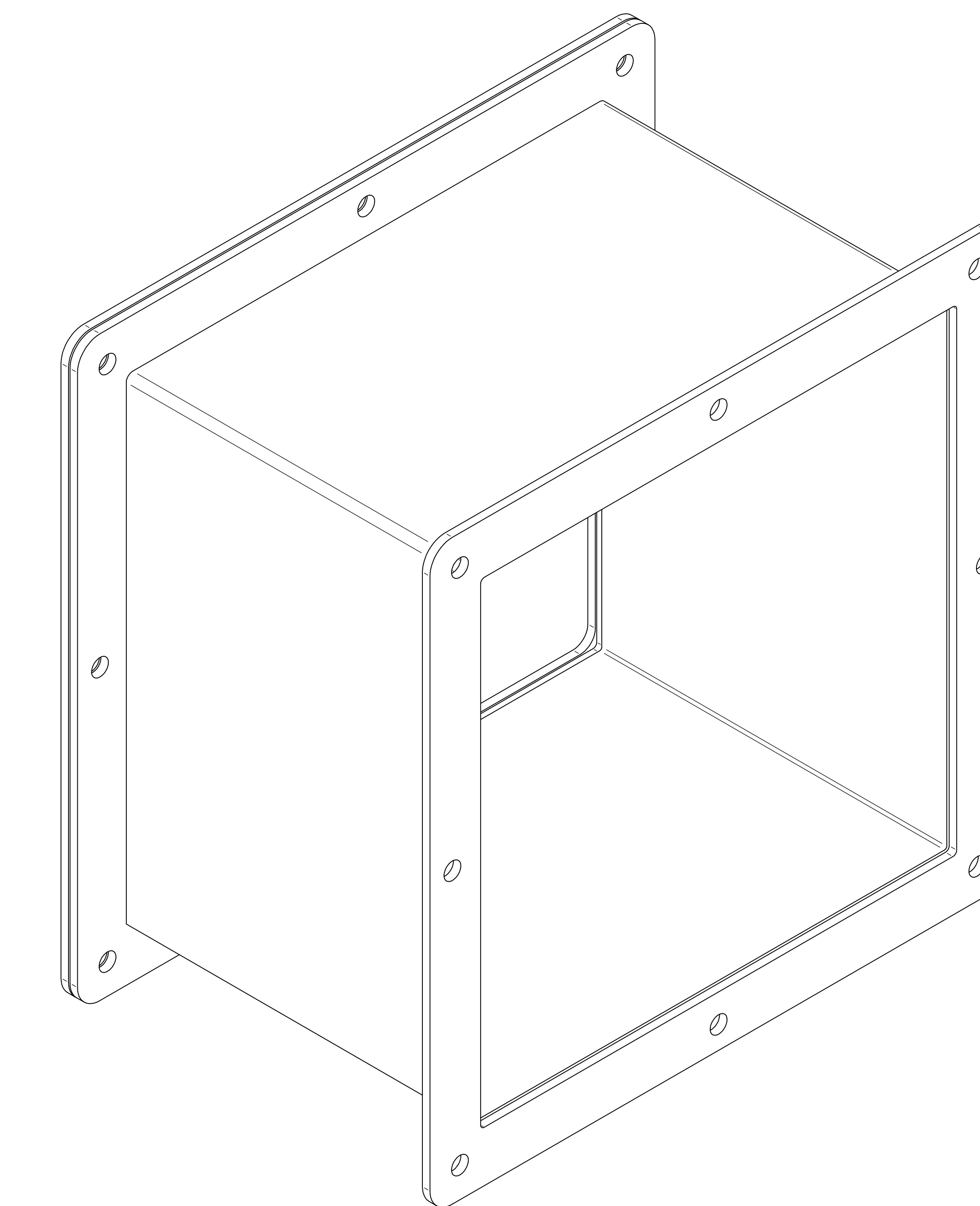
ISOMETRIC VIEWS
