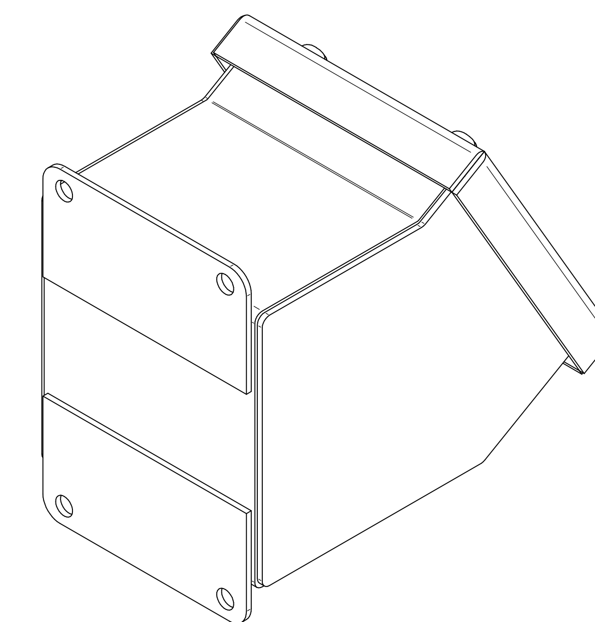
ISOMETRIC VIEWS
