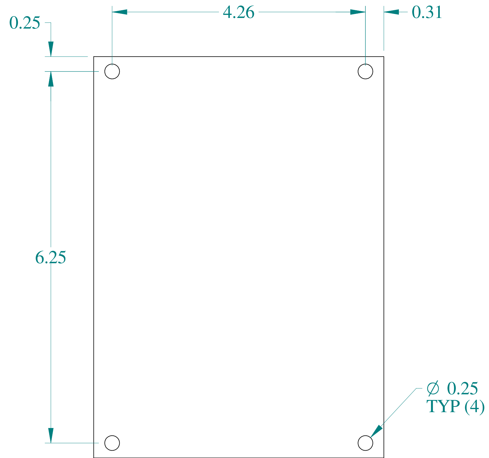
FRONT VIEW
