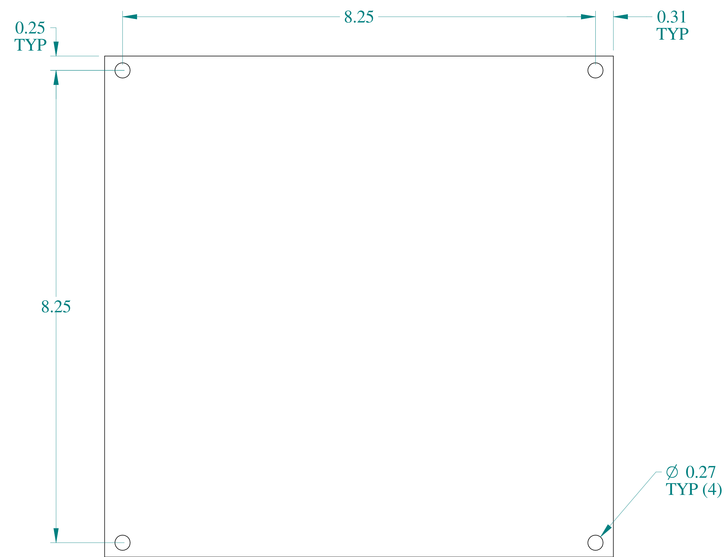
FRONT VIEW
