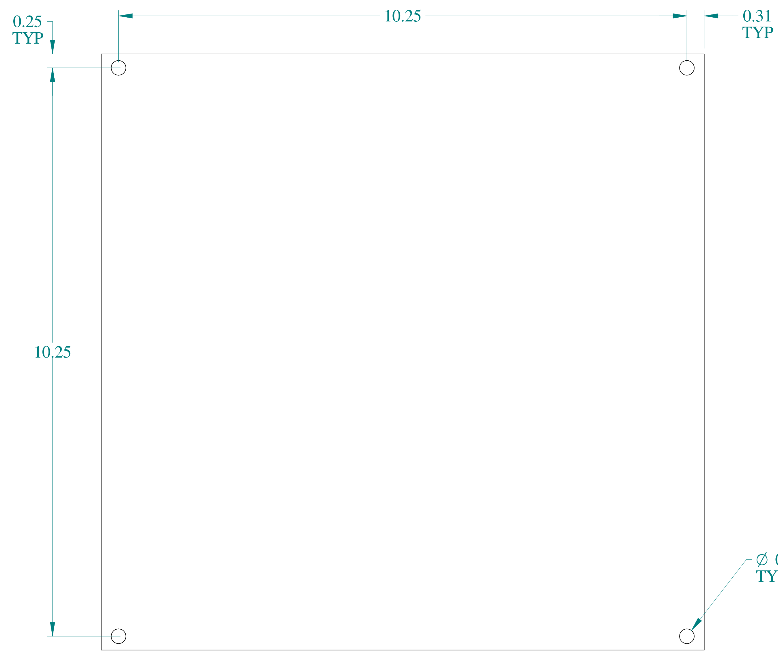
FRONT VIEW
