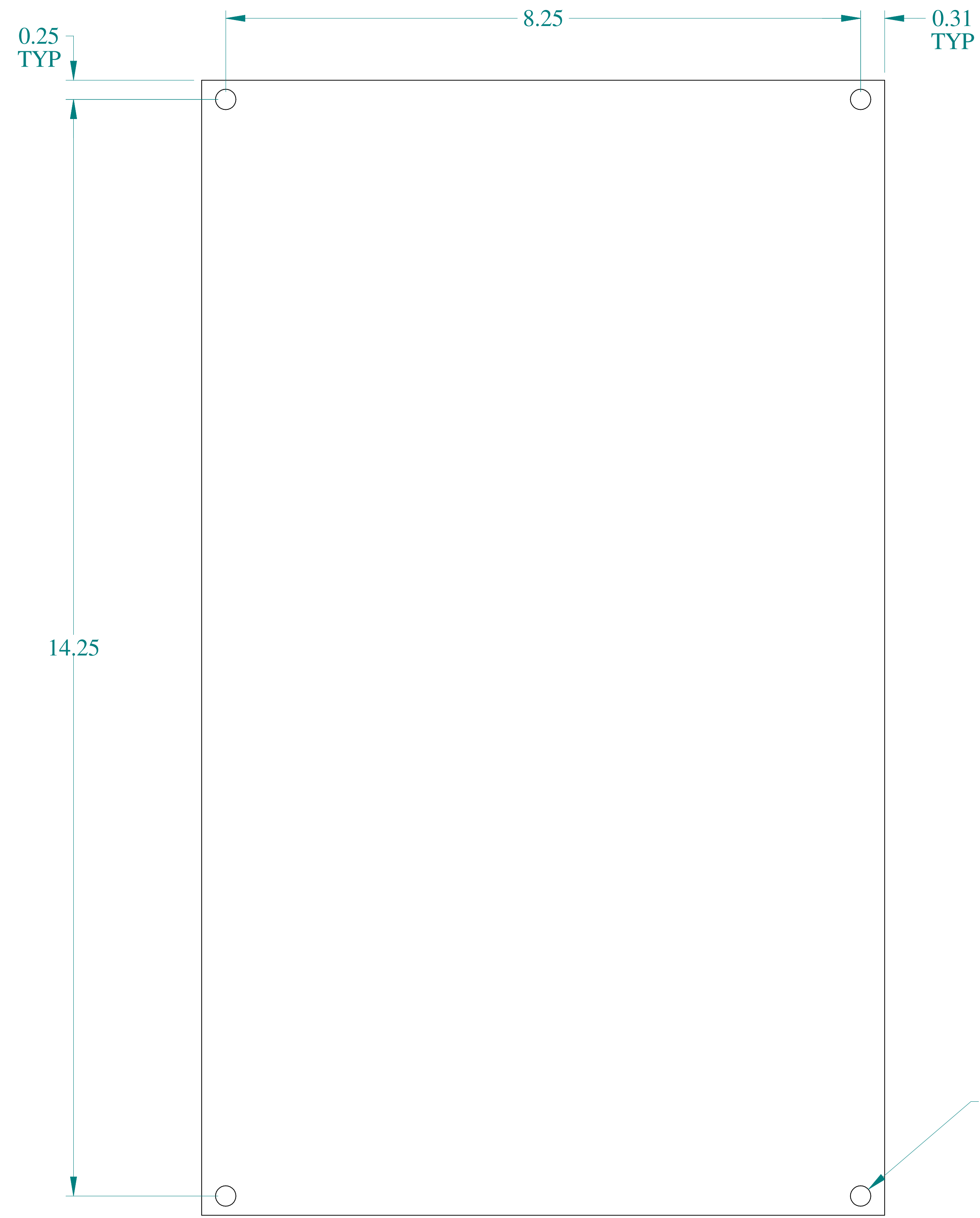
FRONT VIEW
