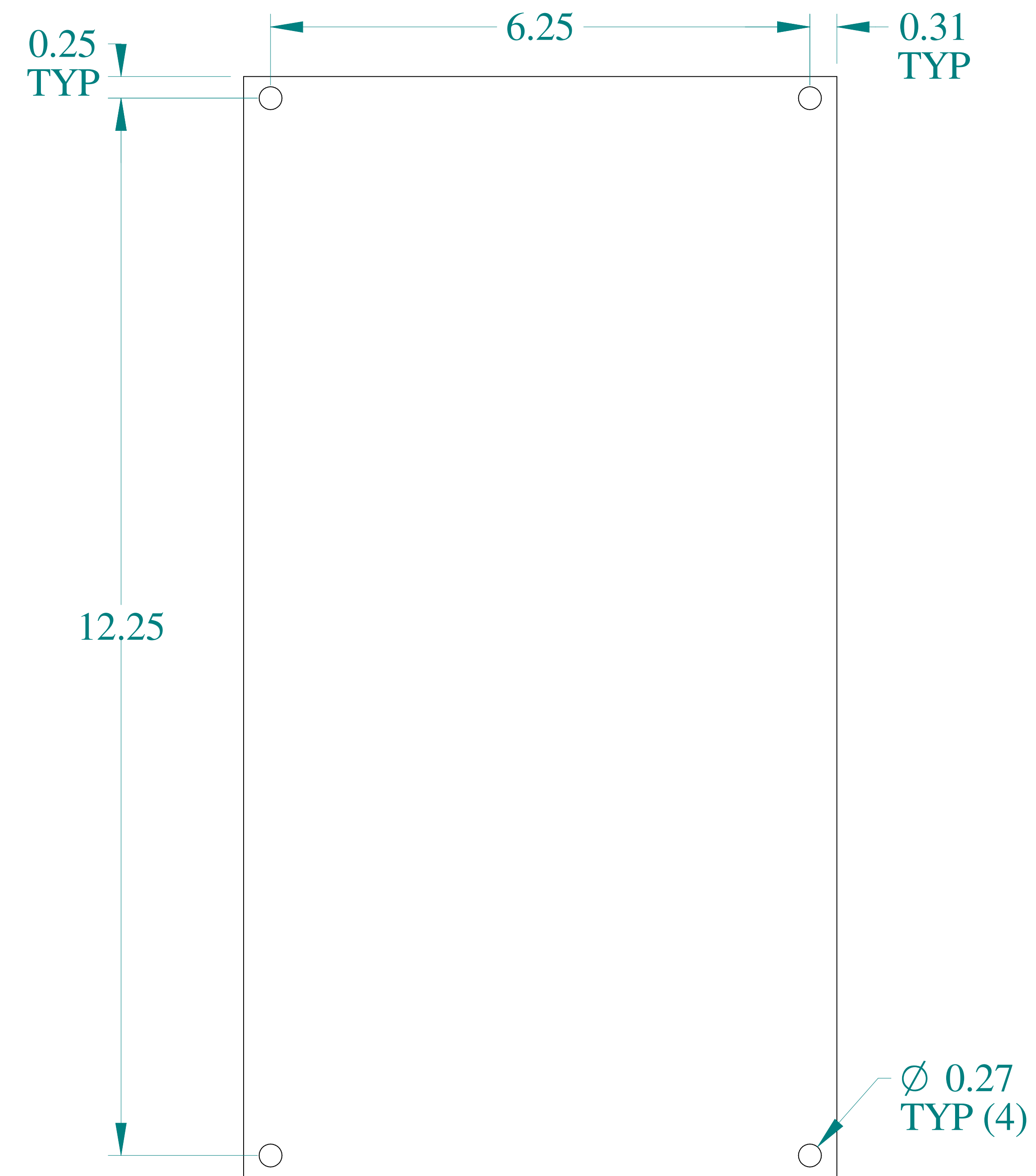
FRONT VIEW
