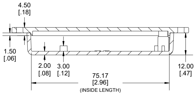
SIDE VIEW SECTION A-A
