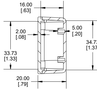
END VIEW SECTION A-A
