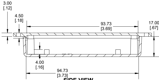
SIDE VIEW SECTION B-B
