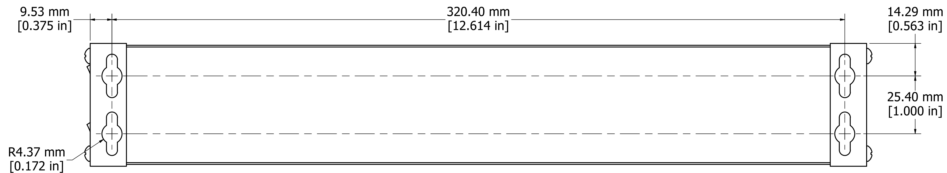
ASSEMBLY - VIEW FROM BOTTOM
