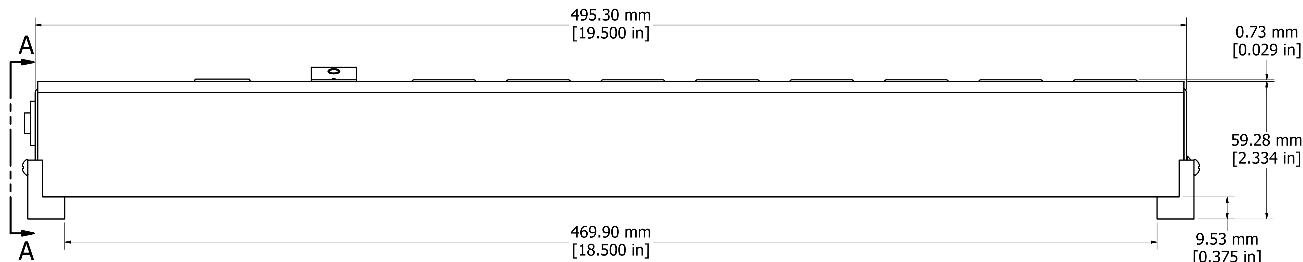
ASSEMBLY - VIEW FROM SIDE
