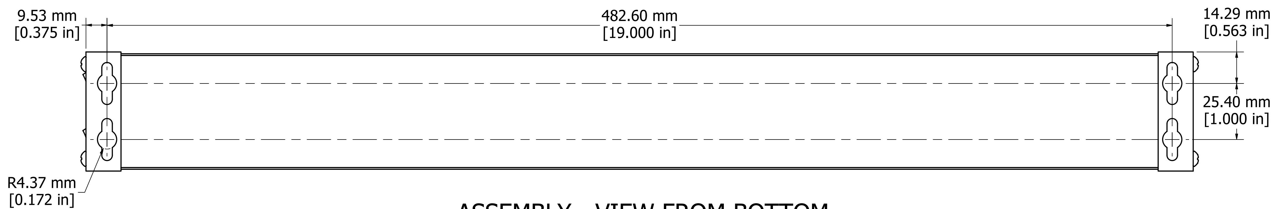
ASSEMBLY - VIEW FROM BOTTOM
