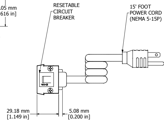
ASSEMBLY - VIEW FROM EMD
