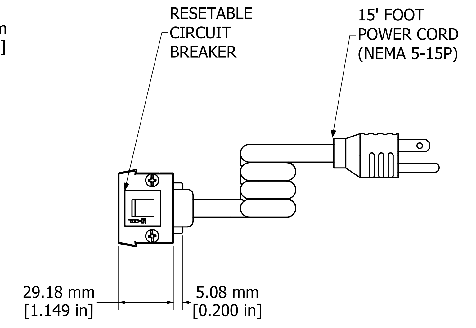
ASSEMBLY - VIEW FROM END
