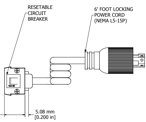
ASSEMBLY - VIEW FROM END
