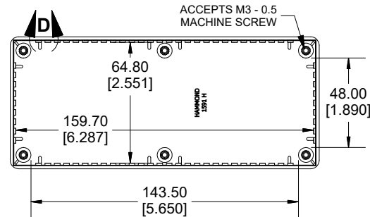
INSIDE BOX
