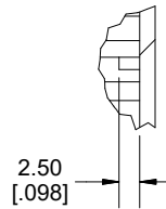
DETAIL C
