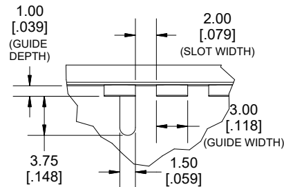
DETAIL D
