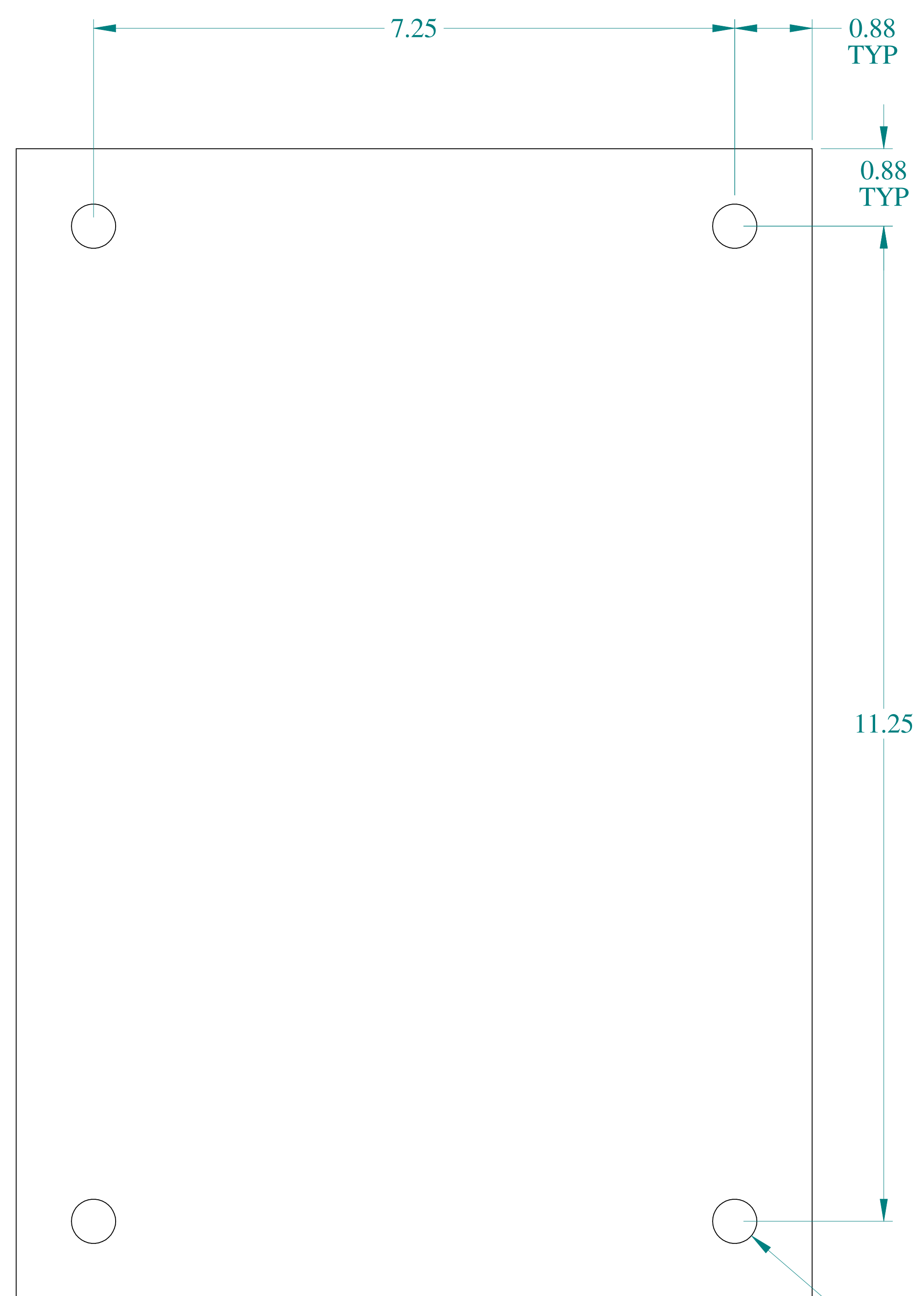
FRONT VIEW
