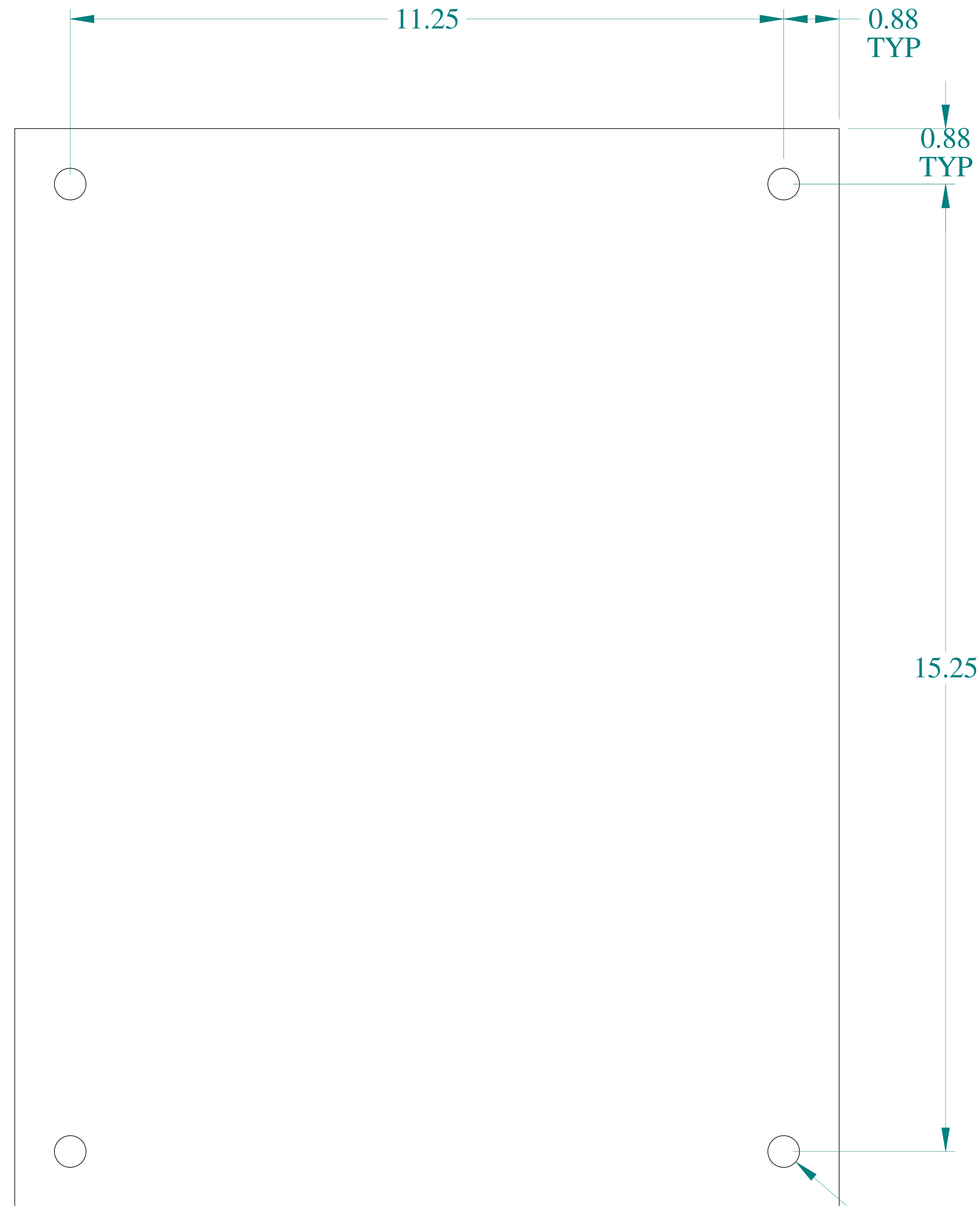
FRONT VIEW
