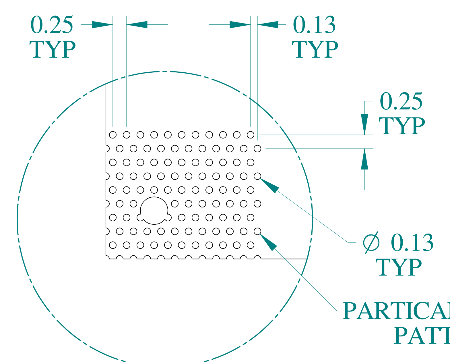
DETAIL Z
