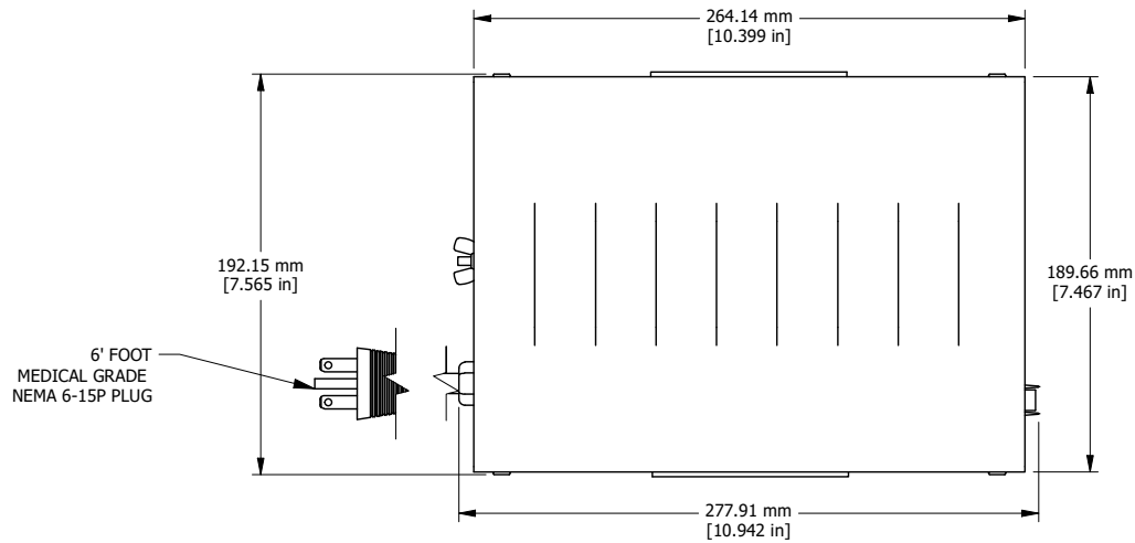
ASSEMBLY - VIEW FROM TOP
