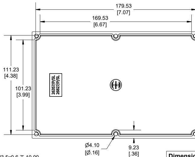
INSIDE LID VIEW
