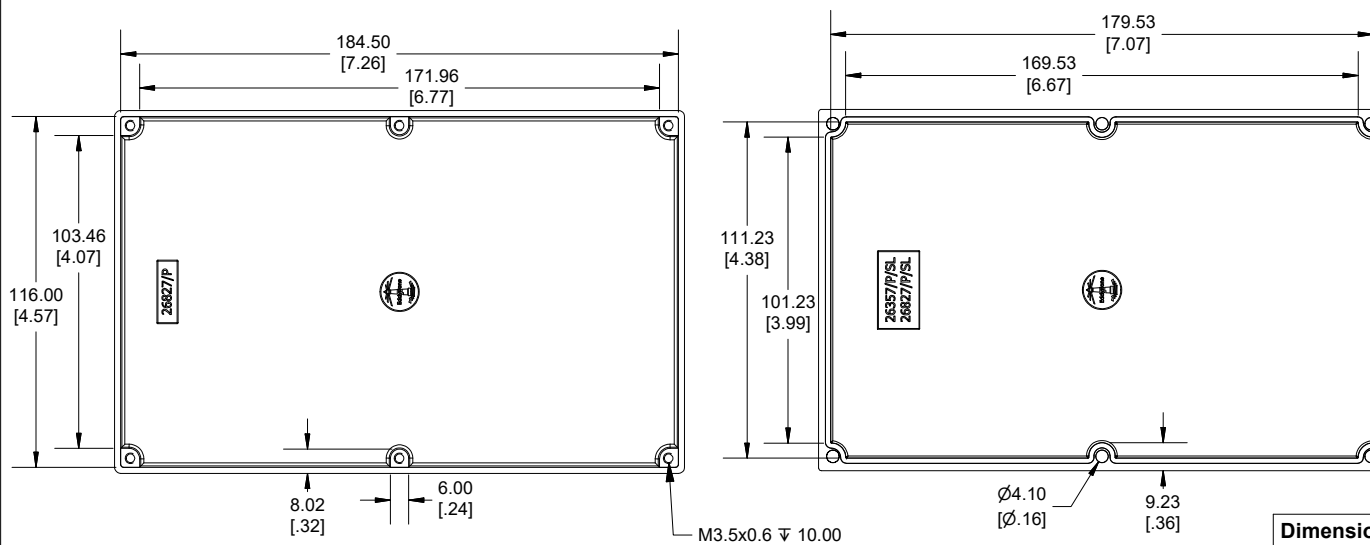
INSIDE BOX VIEW
