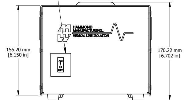
ASSEMBLY - VIEW FROM FRONT
