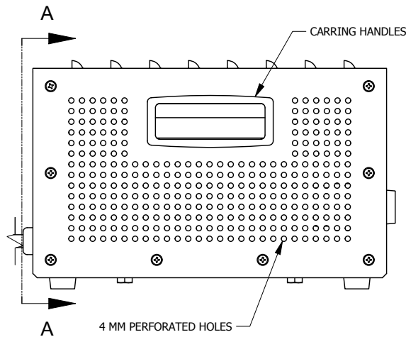
ASSEMBLY - VIEW FROM TOP
