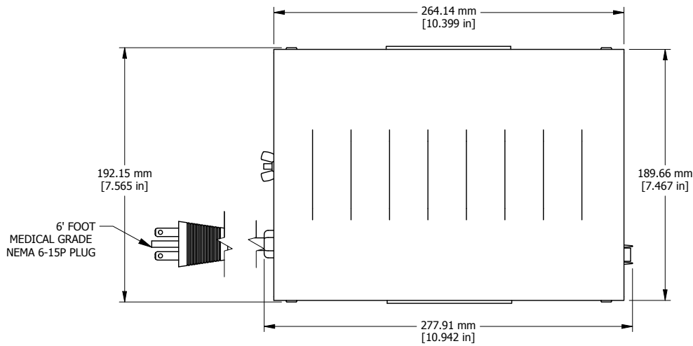
ASSEMBLY - VIEW FROM TOP
