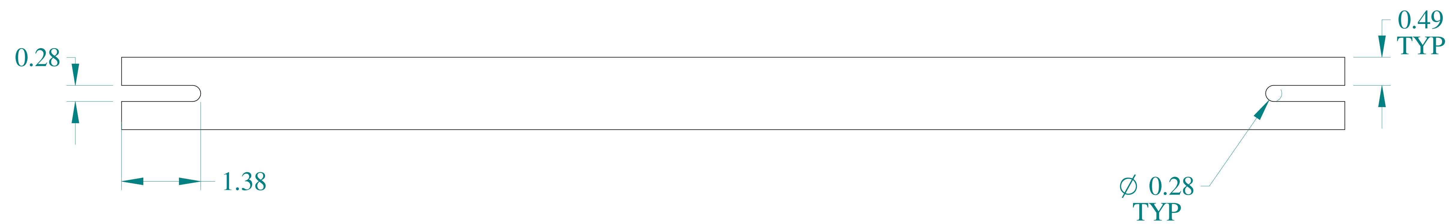
BOTTOM VIEW
