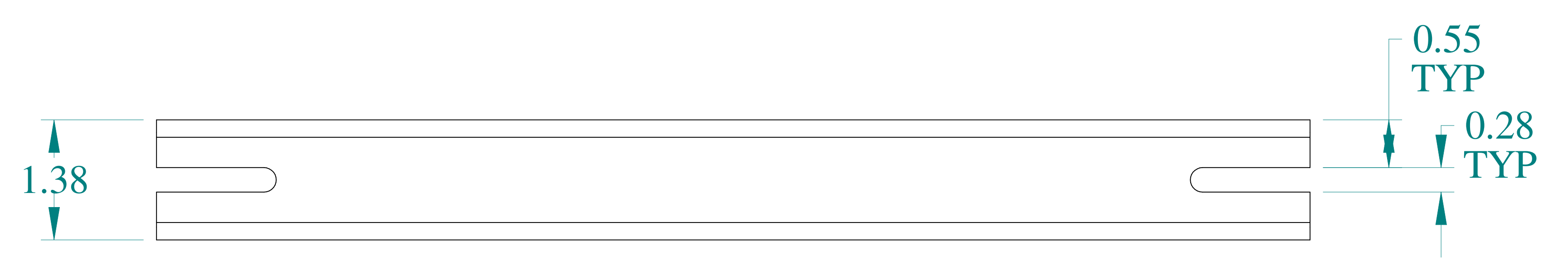
BACK VIEW
