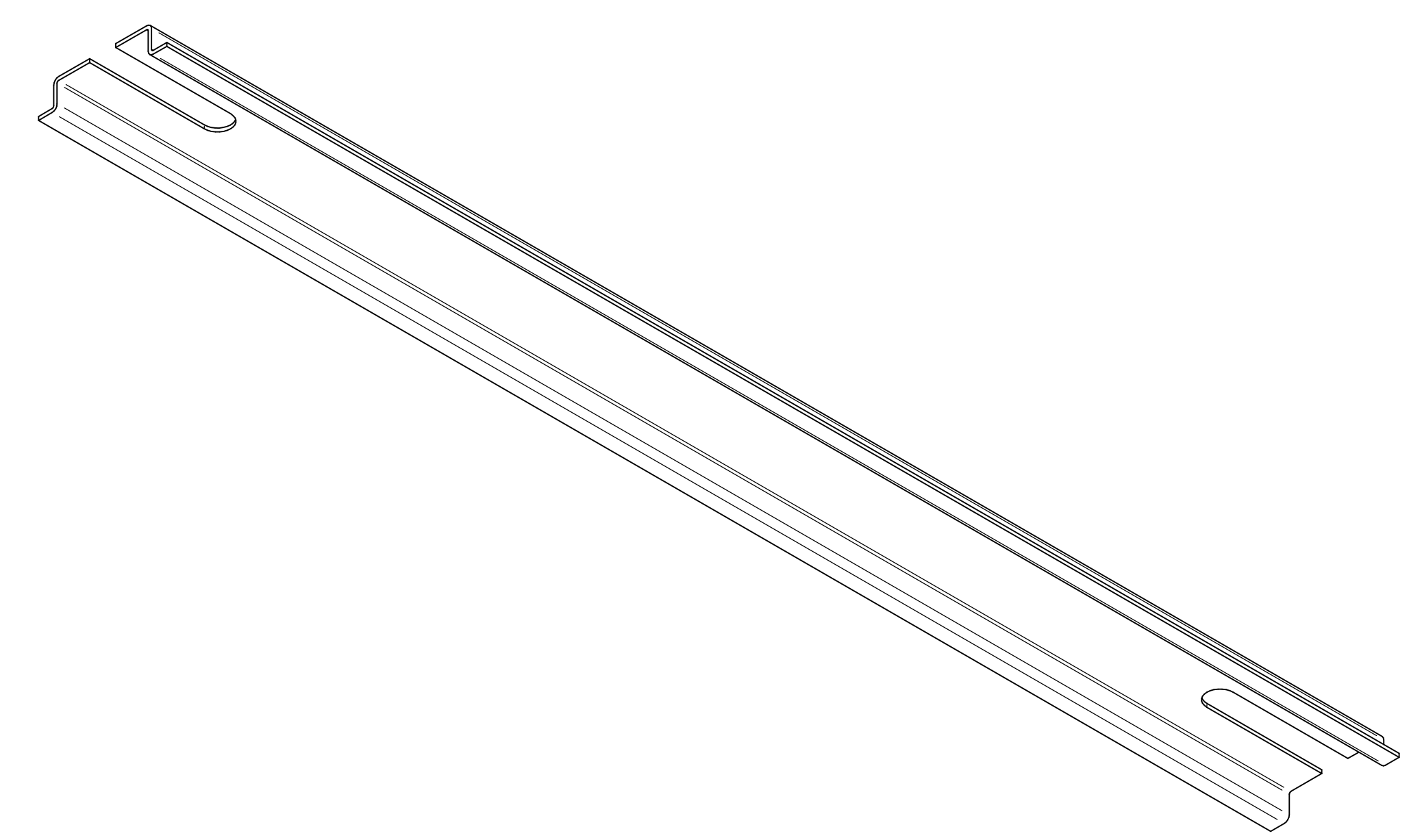
ISOMETRIC VIEWS
