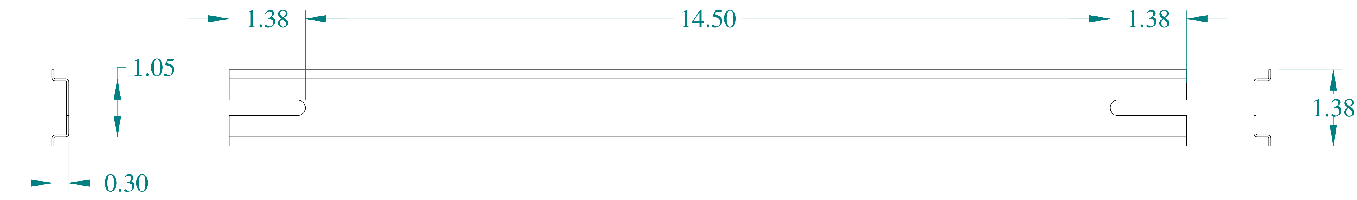
SIDE VIEW
