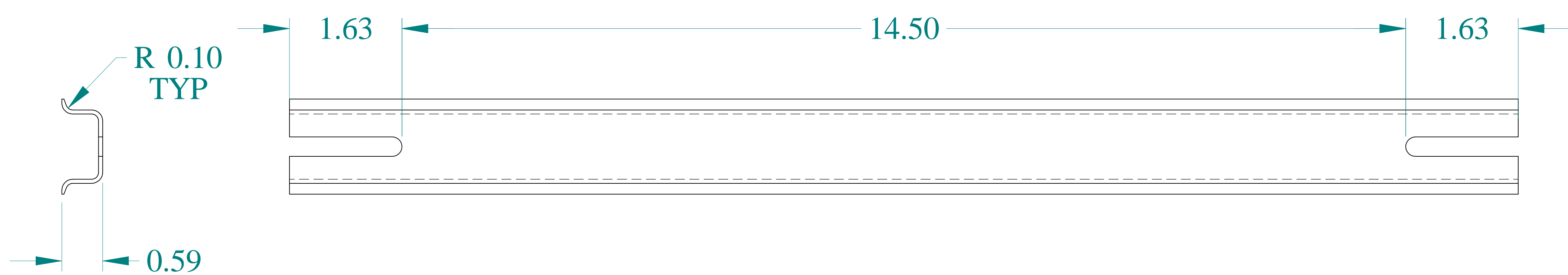
FRONT VIEW
