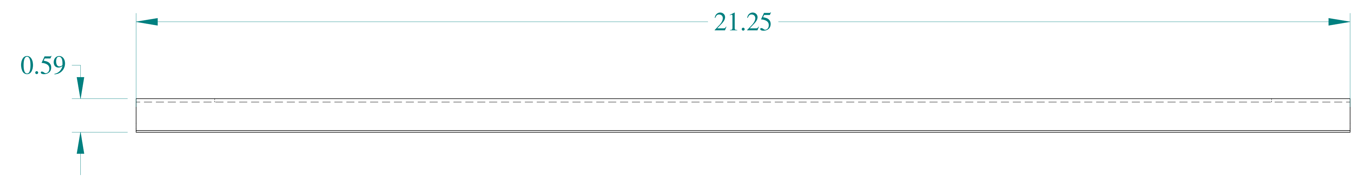
BOTTOM VIEW
