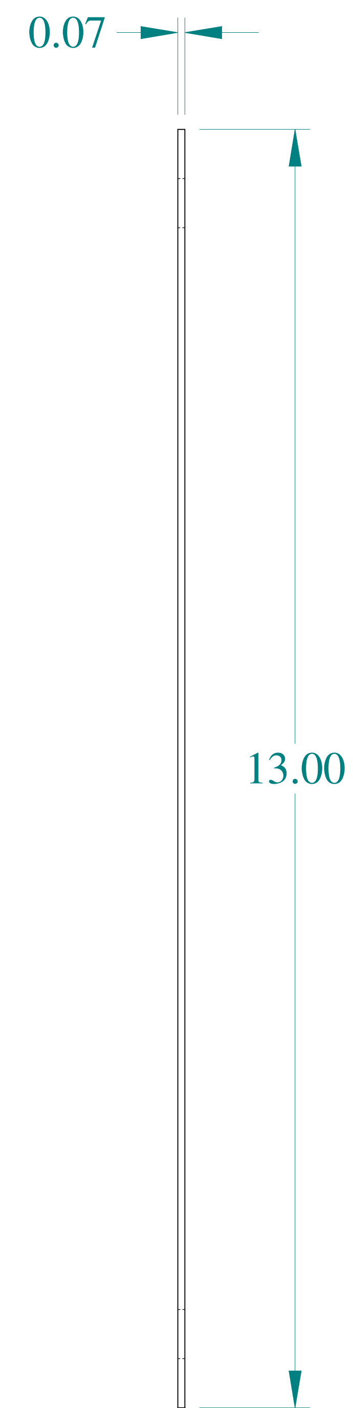
SIDE VIEW
