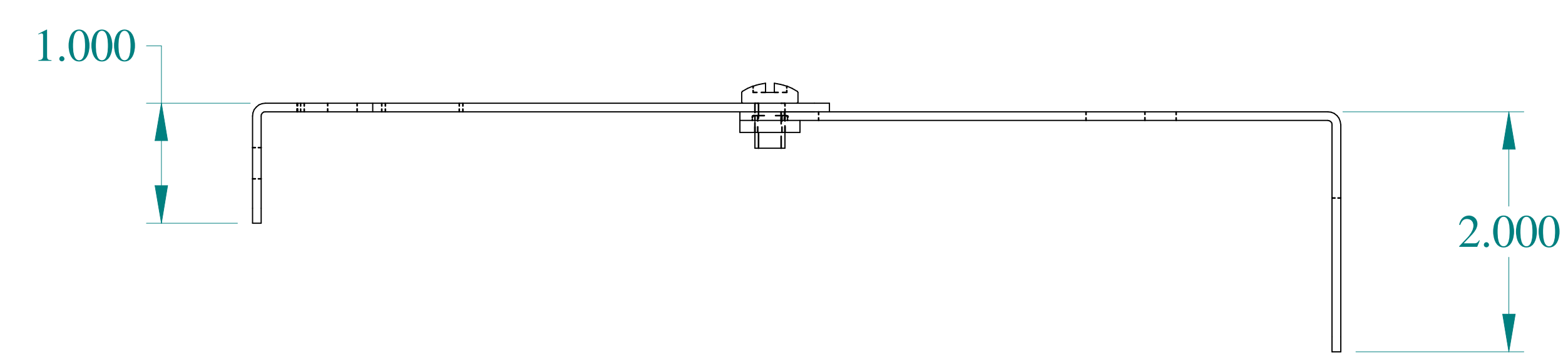
TOP VIEW
