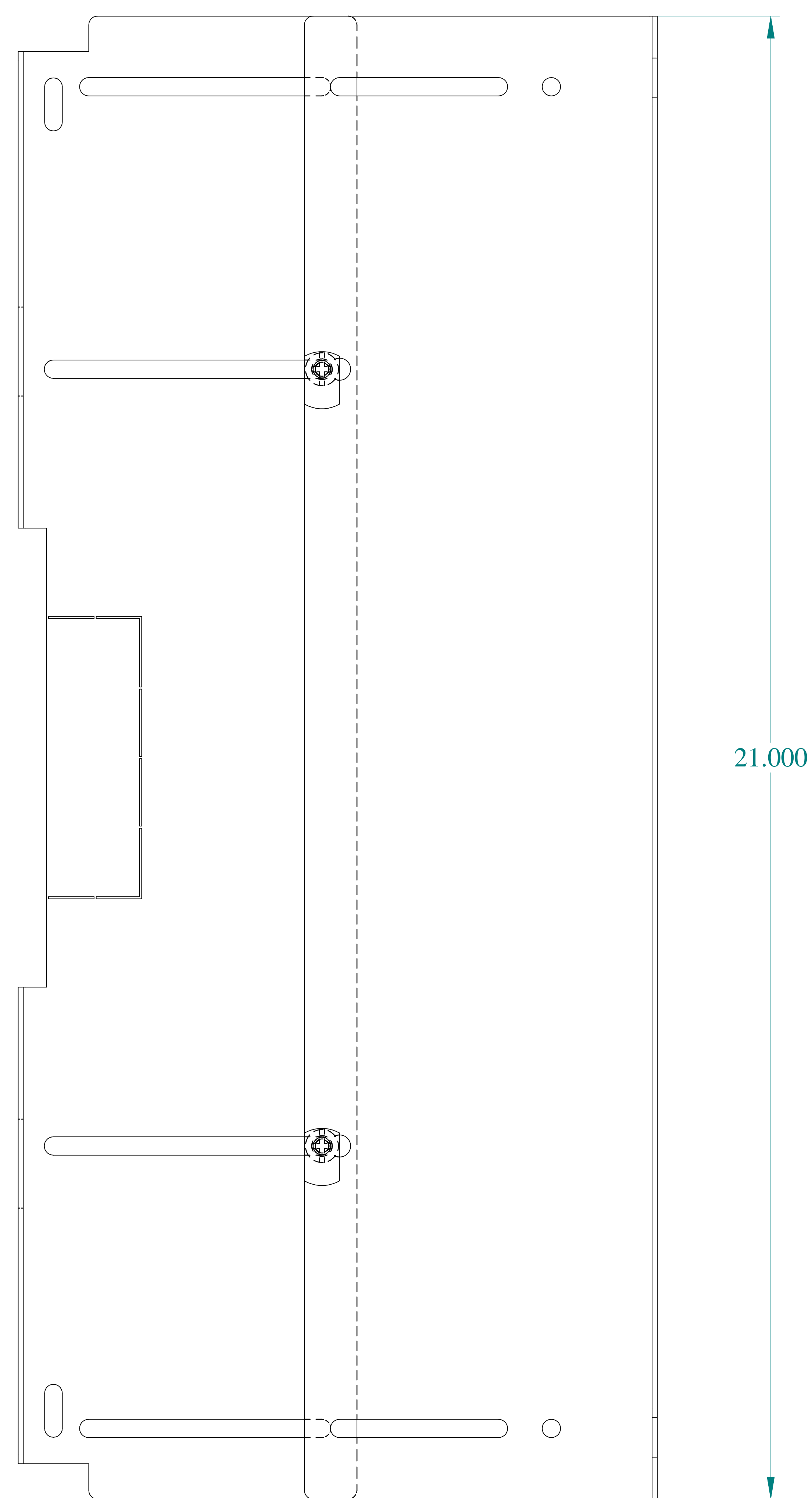
FRONT VIEW
