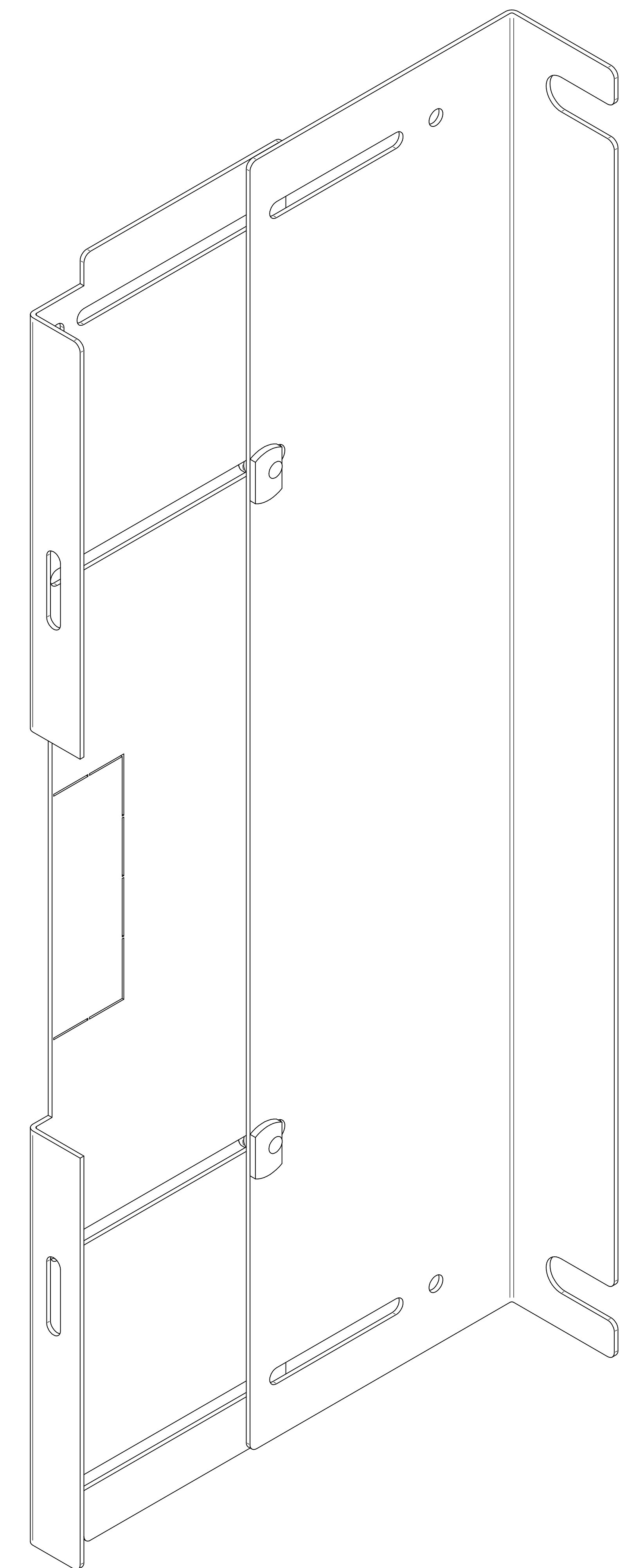
ISOMETRIC VIEW
