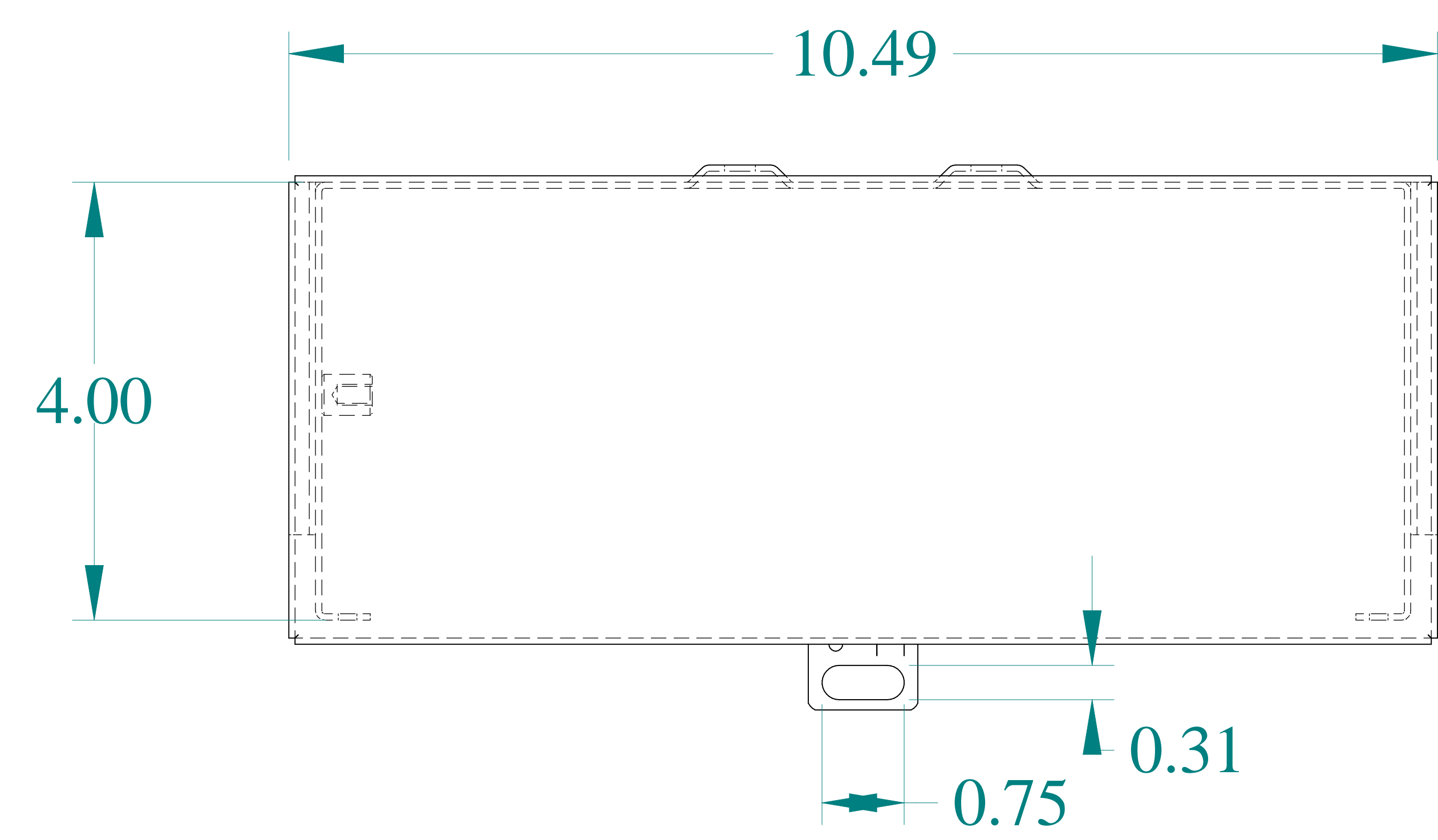
TOP VIEW
