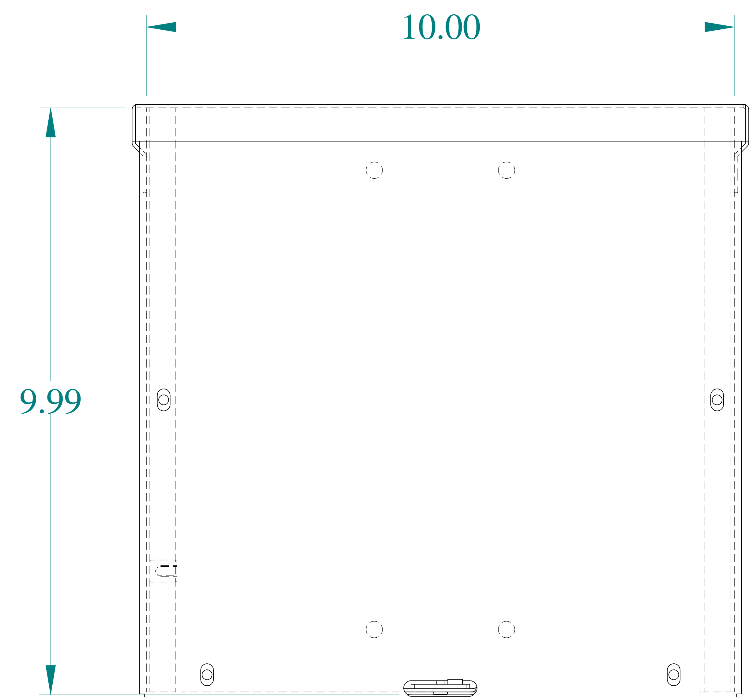
FRONT VIEW
