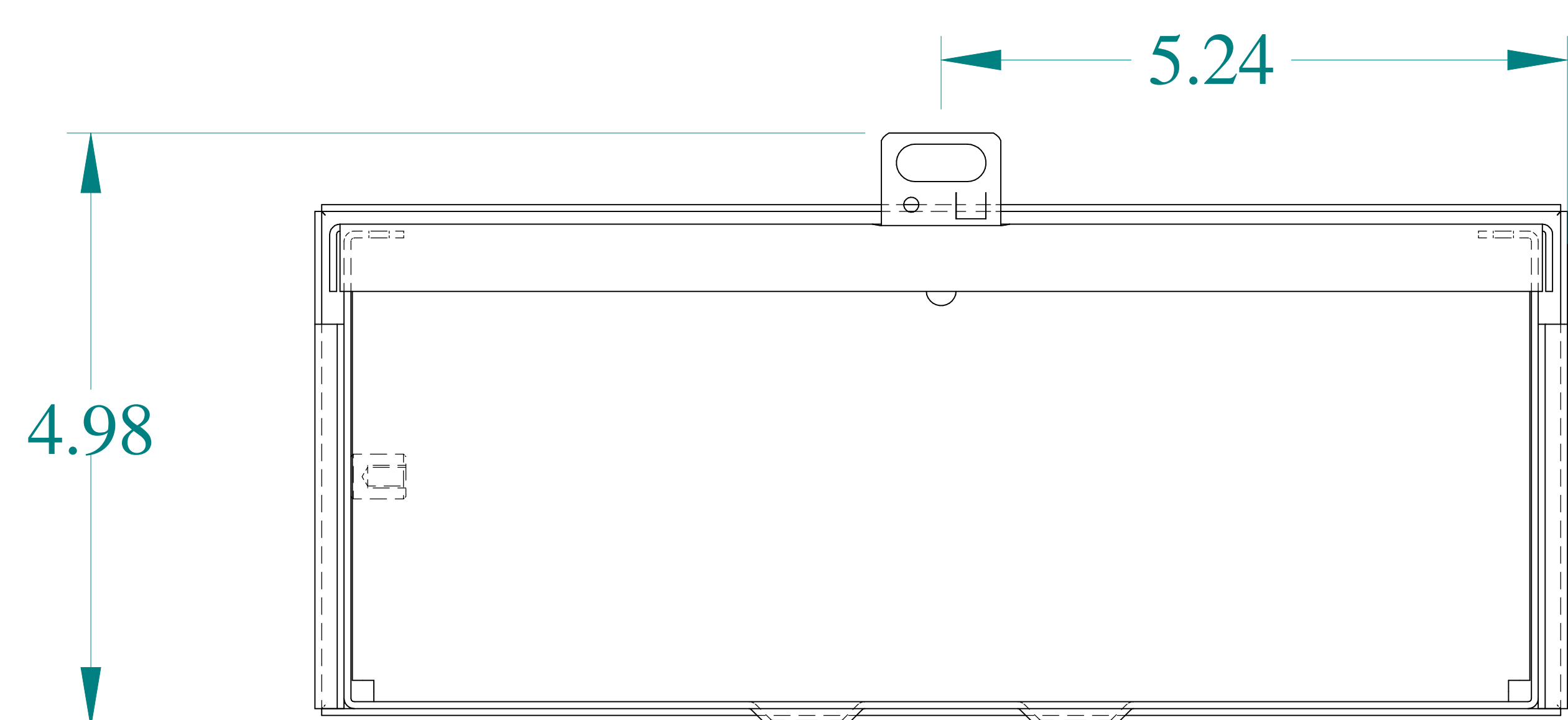
BOTTOM VIEW
